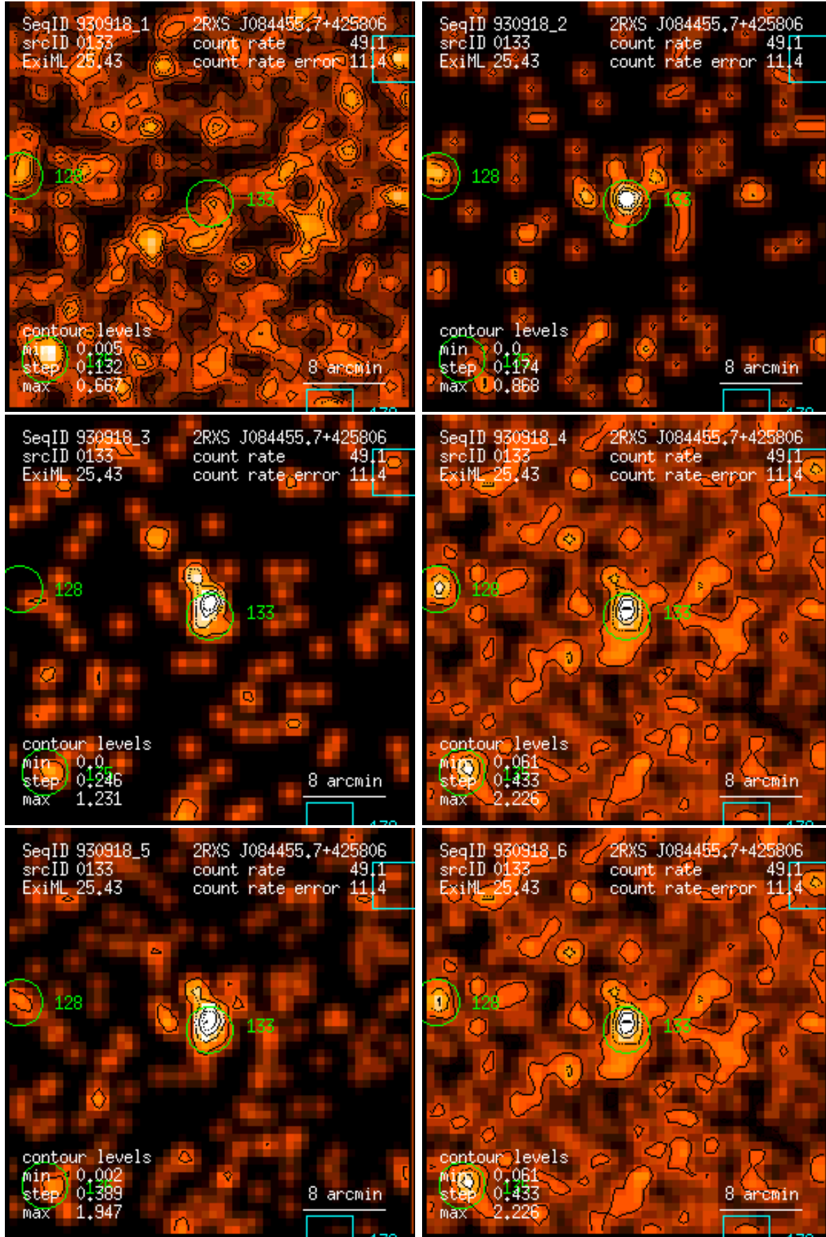
Figure 133: RASS 930918: detection 0133: band rate images, Gaussian filter: (1) PSPC channels 11 – 41, (2) 52 – 90, (3) 91 – 201, (4) 11 – 235, (5) 52 – 201, (6) 11 – 201. Broad band rates in counts/ks. Band rate contour levels in counts/ks/arcmin 2 .
