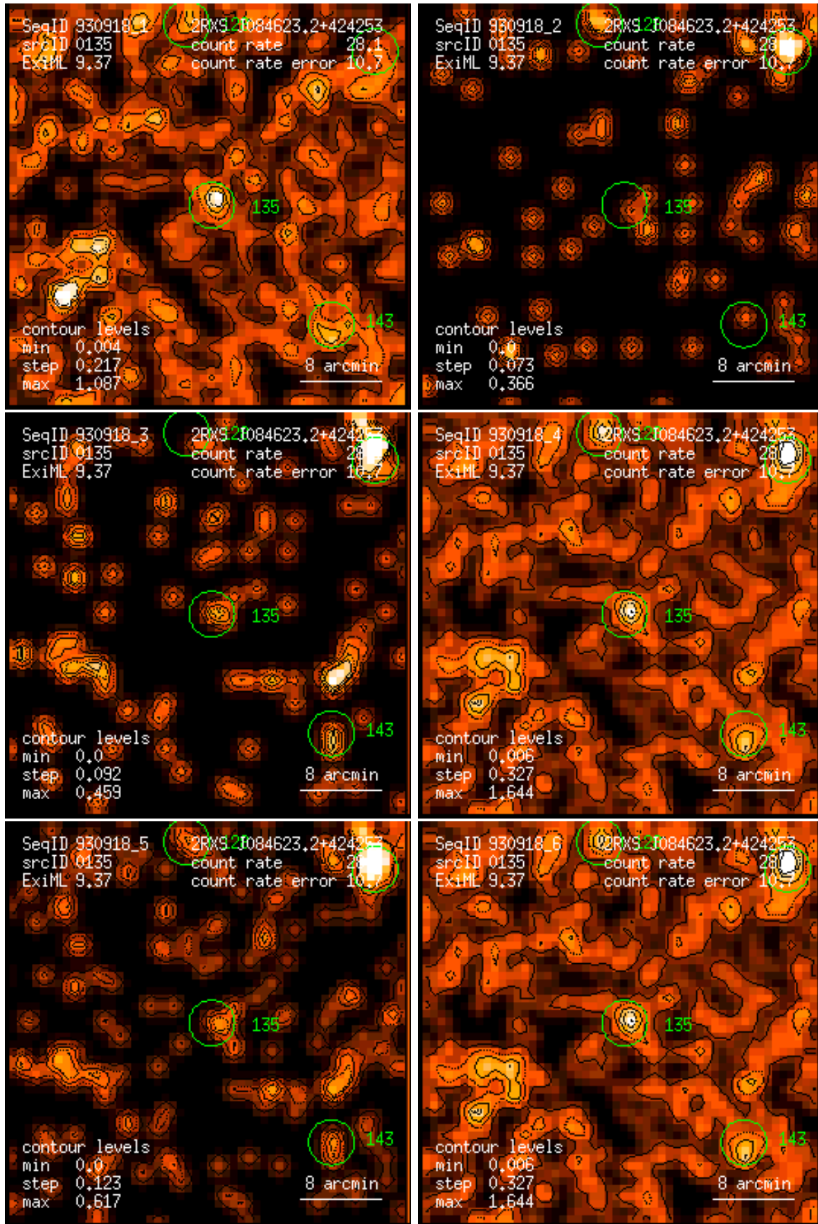
Figure 135: RASS 930918: detection 0135: band rate images, Gaussian filter: (1) PSPC channels 11 – 41, (2) 52 – 90, (3) 91 – 201, (4) 11 – 235, (5) 52 – 201, (6) 11 – 201. Broad band rates in counts/ks. Band rate contour levels in counts/ks/arcmin 2 .
