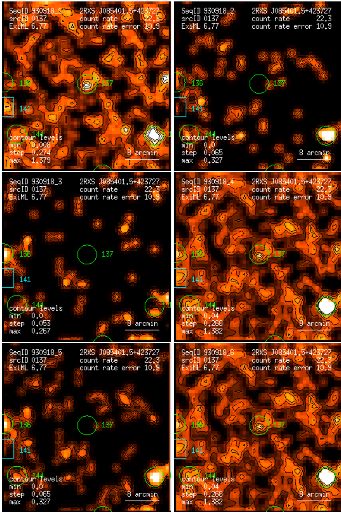
Figure 137: RASS 930918: detection 0137: band rate images, Gaussian filter: (1) PSPC channels 11 – 41, (2) 52 – 90, (3) 91 – 201, (4) 11 – 235, (5) 52 – 201, (6) 11 – 201. Broad band rates in counts/ks. Band rate contour levels in counts/ks/arcmin 2 .
