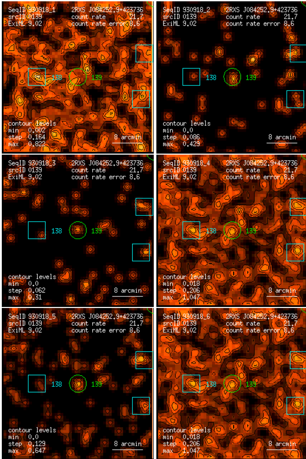
Figure 139: RASS 930918: detection 0139: band rate images, Gaussian filter: (1) PSPC channels 11 – 41, (2) 52 – 90, (3) 91 – 201, (4) 11 – 235, (5) 52 – 201, (6) 11 – 201. Broad band rates in counts/ks. Band rate contour levels in counts/ks/arcmin 2 .
