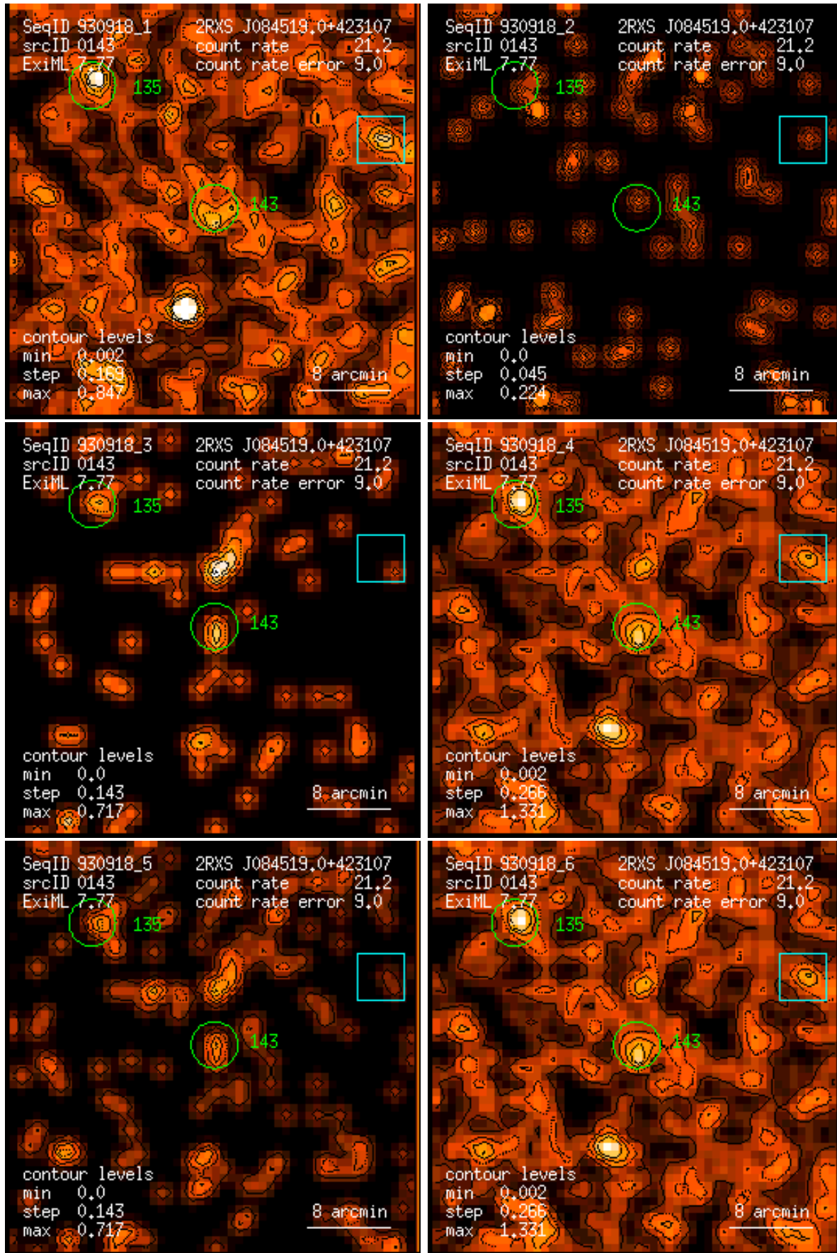
Figure 143: RASS 930918: detection 0143: band rate images, Gaussian filter: (1) PSPC channels 11 – 41, (2) 52 – 90, (3) 91 – 201, (4) 11 – 235, (5) 52 – 201, (6) 11 – 201. Broad band rates in counts/ks. Band rate contour levels in counts/ks/arcmin 2 .
