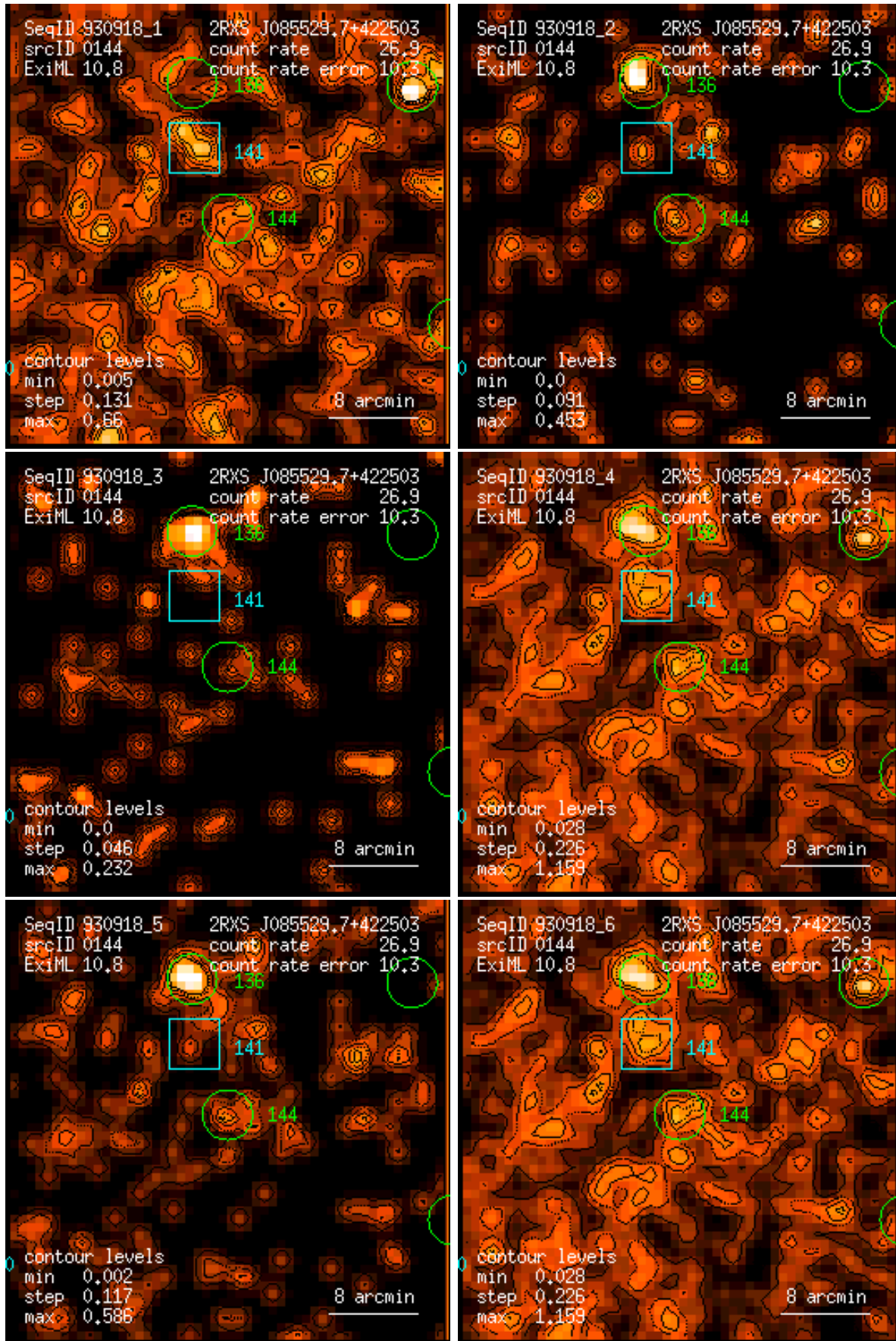
Figure 144: RASS 930918: detection 0144: band rate images, Gaussian filter: (1) PSPC channels 11 – 41, (2) 52 – 90, (3) 91 – 201, (4) 11 – 235, (5) 52 – 201, (6) 11 – 201. Broad band rates in counts/ks. Band rate contour levels in counts/ks/arcmin 2 .
