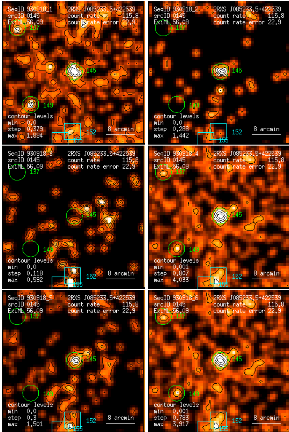
Figure 145: RASS 930918: detection 0145: band rate images, Gaussian filter: (1) PSPC channels 11 – 41, (2) 52 – 90, (3) 91 – 201, (4) 11 – 235, (5) 52 – 201, (6) 11 – 201. Broad band rates in counts/ks. Band rate contour levels in counts/ks/arcmin 2 .
