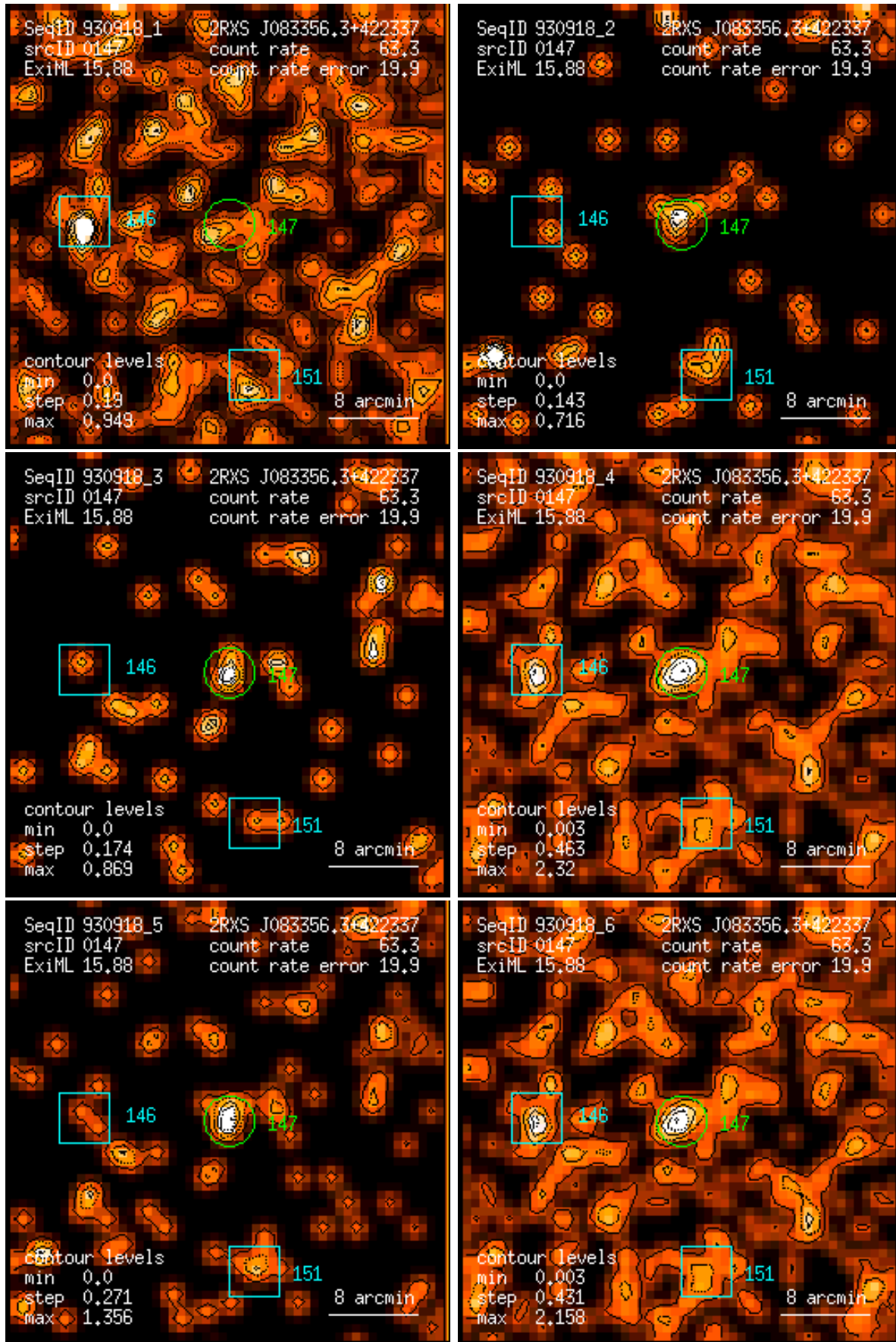
Figure 147: RASS 930918: detection 0147: band rate images, Gaussian filter: (1) PSPC channels 11 – 41, (2) 52 – 90, (3) 91 – 201, (4) 11 – 235, (5) 52 – 201, (6) 11 – 201. Broad band rates in counts/ks. Band rate contour levels in counts/ks/arcmin 2 .
