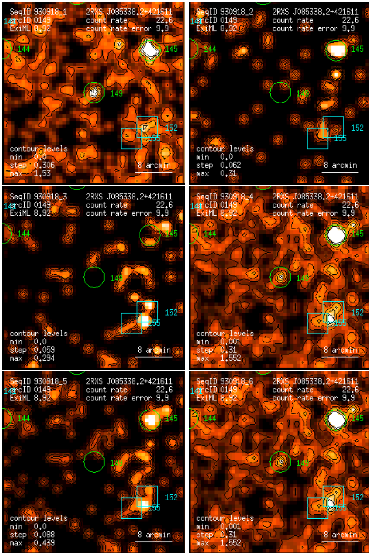
Figure 149: RASS 930918: detection 0149: band rate images, Gaussian filter: (1) PSPC channels 11 – 41, (2) 52 – 90, (3) 91 – 201, (4) 11 – 235, (5) 52 – 201, (6) 11 – 201. Broad band rates in counts/ks. Band rate contour levels in counts/ks/arcmin 2 .
