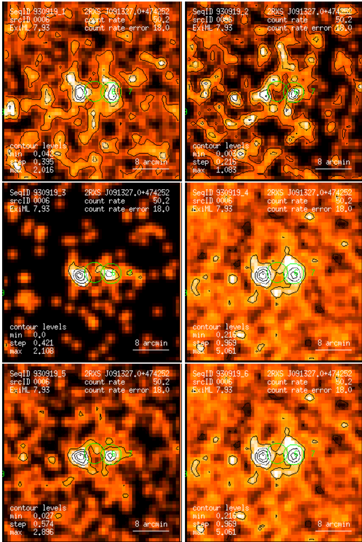
Figure 6: RASS 930919: detection 0006: band rate images, Gaussian filter: (1) PSPC channels 11 – 41, (2) 52 – 90, (3) 91 – 201, (4) 11 – 235, (5) 52 – 201, (6) 11 – 201. Broad band rates in counts/ks. Band rate contour levels in counts/ks/arcmin 2 .
