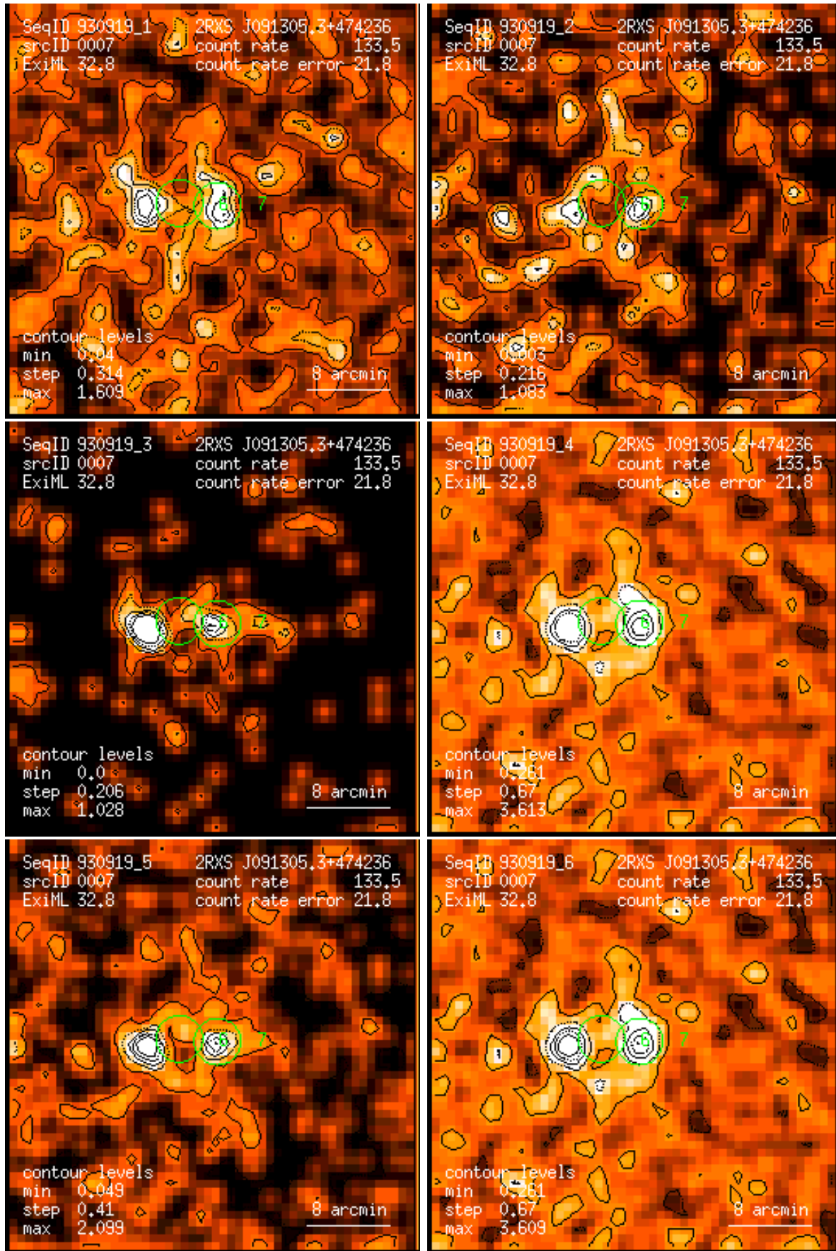
Figure 7: RASS 930919: detection 0007: band rate images, Gaussian filter: (1) PSPC channels 11 – 41, (2) 52 – 90, (3) 91 – 201, (4) 11 – 235, (5) 52 – 201, (6) 11 – 201. Broad band rates in counts/ks. Band rate contour levels in counts/ks/arcmin 2 .
