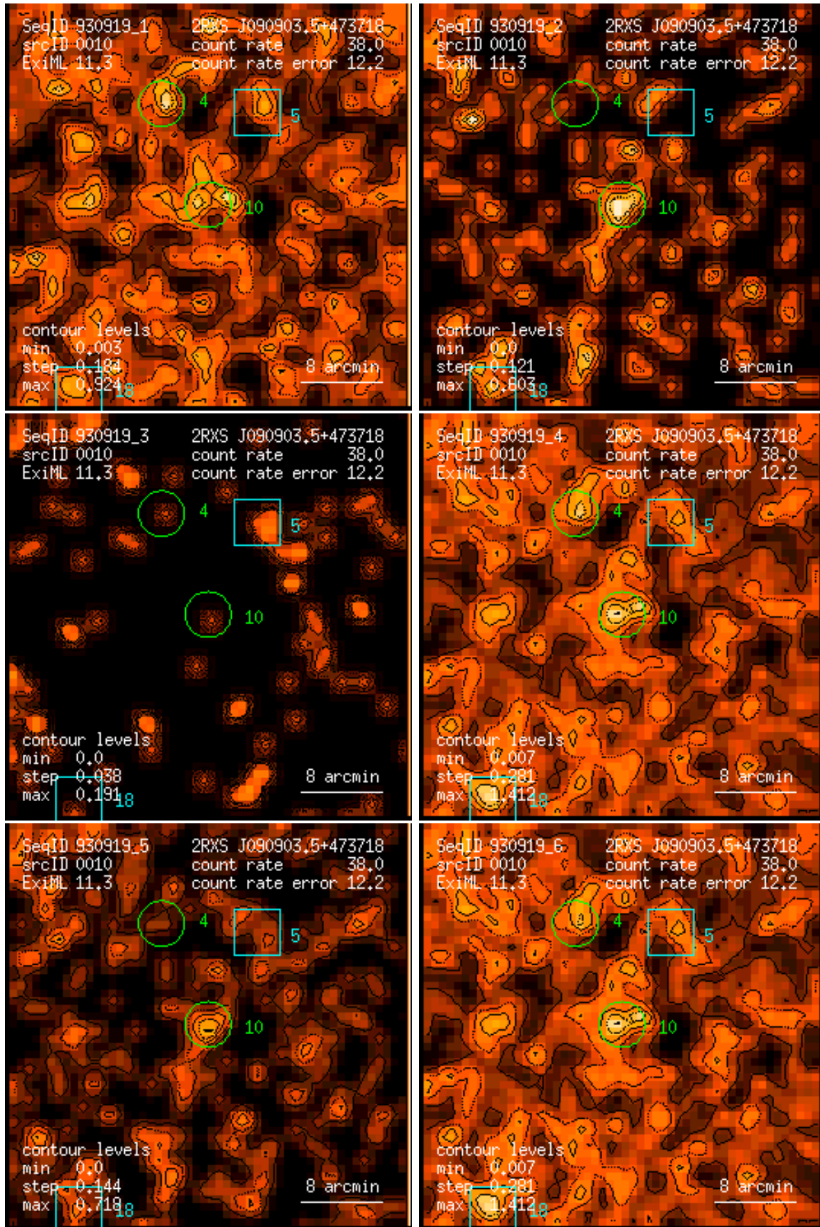
Figure 10: RASS 930919: detection 0010: band rate images, Gaussian filter: (1) PSPC channels 11 – 41, (2) 52 – 90, (3) 91 – 201, (4) 11 – 235, (5) 52 – 201, (6) 11 – 201. Broad band rates in counts/ks. Band rate contour levels in counts/ks/arcmin 2 .
