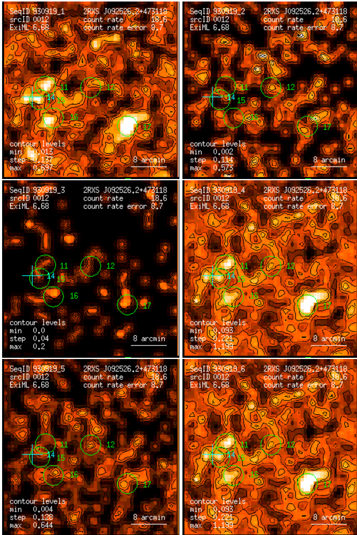
Figure 12: RASS 930919: detection 0012: band rate images, Gaussian filter: (1) PSPC channels 11 – 41, (2) 52 – 90, (3) 91 – 201, (4) 11 – 235, (5) 52 – 201, (6) 11 – 201. Broad band rates in counts/ks. Band rate contour levels in counts/ks/arcmin 2 .
