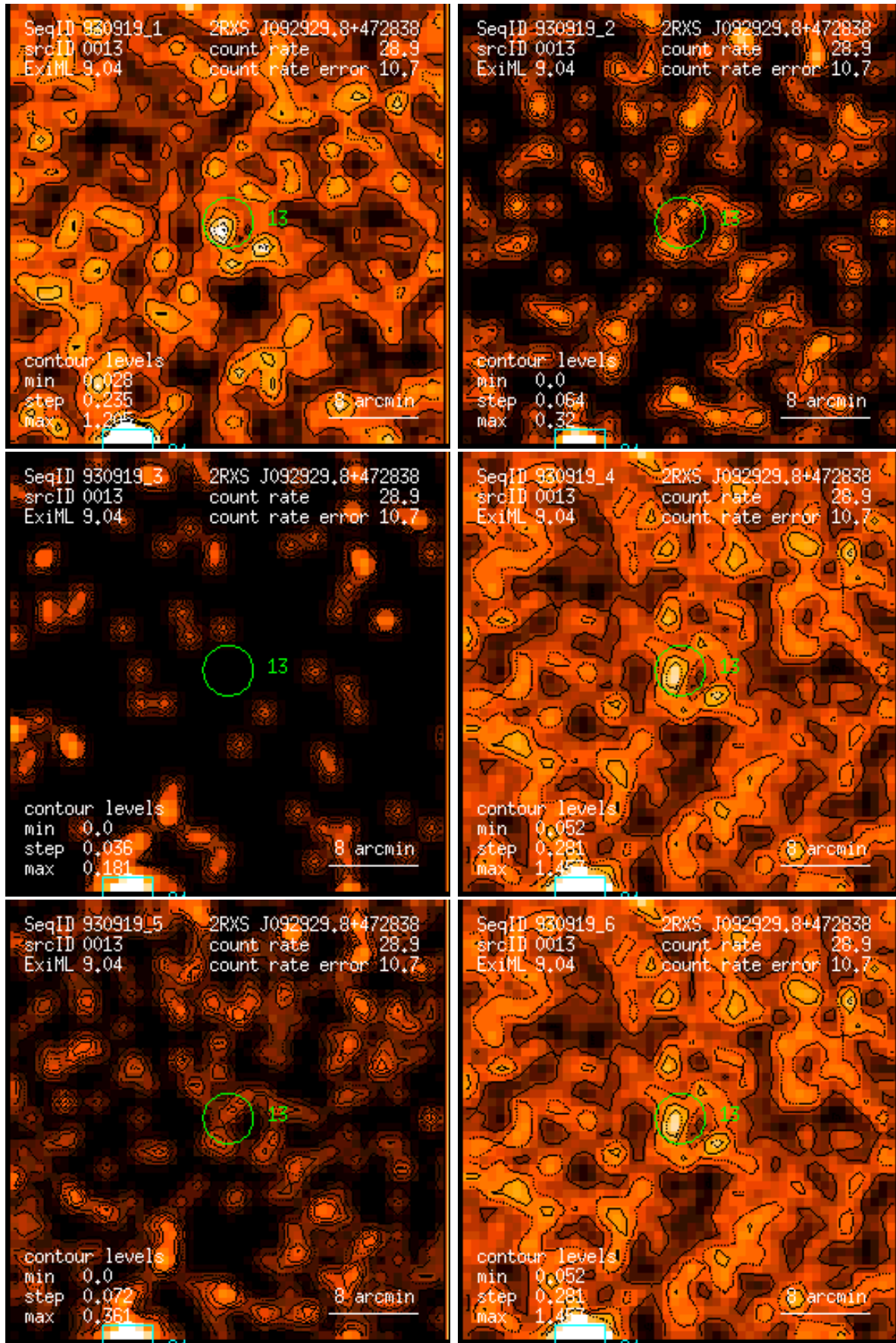
Figure 13: RASS 930919: detection 0013: band rate images, Gaussian filter: (1) PSPC channels 11 – 41, (2) 52 – 90, (3) 91 – 201, (4) 11 – 235, (5) 52 – 201, (6) 11 – 201. Broad band rates in counts/ks. Band rate contour levels in counts/ks/arcmin 2 .
