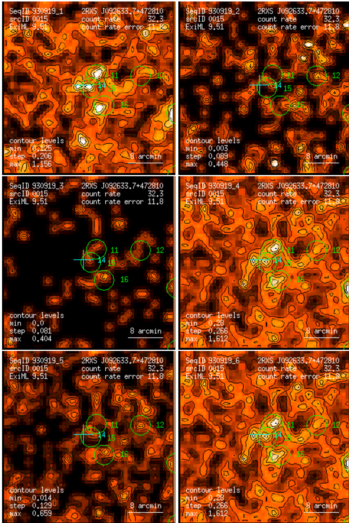
Figure 15: RASS 930919: detection 0015: band rate images, Gaussian filter: (1) PSPC channels 11 – 41, (2) 52 – 90, (3) 91 – 201, (4) 11 – 235, (5) 52 – 201, (6) 11 – 201. Broad band rates in counts/ks. Band rate contour levels in counts/ks/arcmin 2 .
