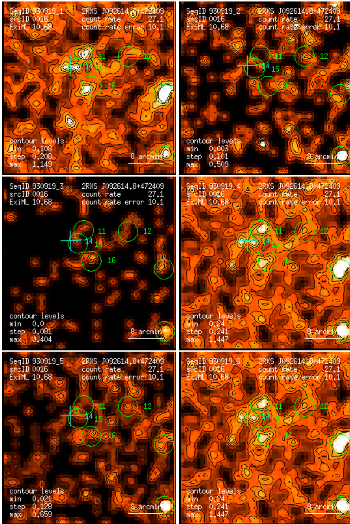
Figure 16: RASS 930919: detection 0016: band rate images, Gaussian filter: (1) PSPC channels 11 – 41, (2) 52 – 90, (3) 91 – 201, (4) 11 – 235, (5) 52 – 201, (6) 11 – 201. Broad band rates in counts/ks. Band rate contour levels in counts/ks/arcmin 2 .
