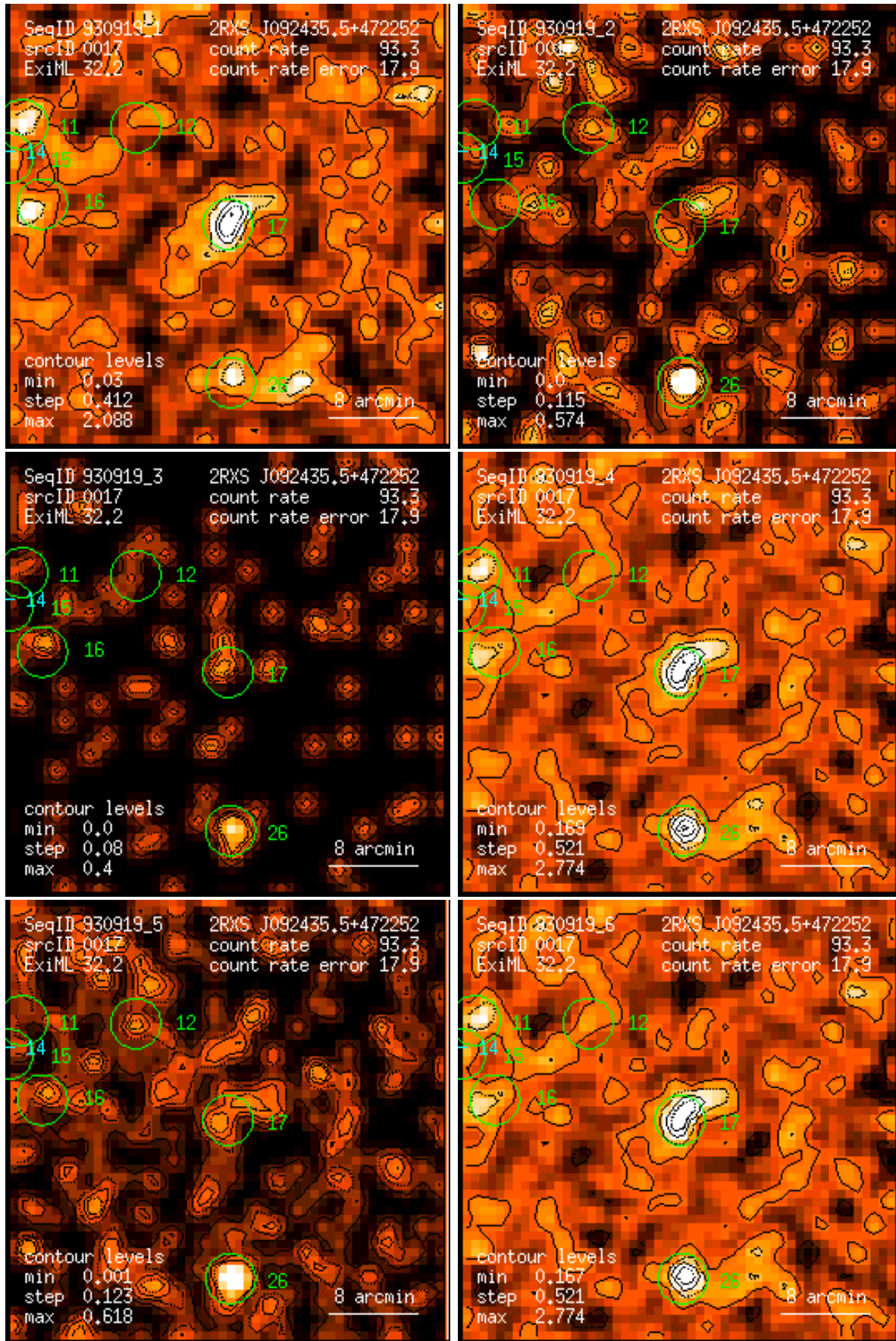
Figure 17: RASS 930919: detection 0017: band rate images, Gaussian filter: (1) PSPC channels 11 – 41, (2) 52 – 90, (3) 91 – 201, (4) 11 – 235, (5) 52 – 201, (6) 11 – 201. Broad band rates in counts/ks. Band rate contour levels in counts/ks/arcmin 2 .
