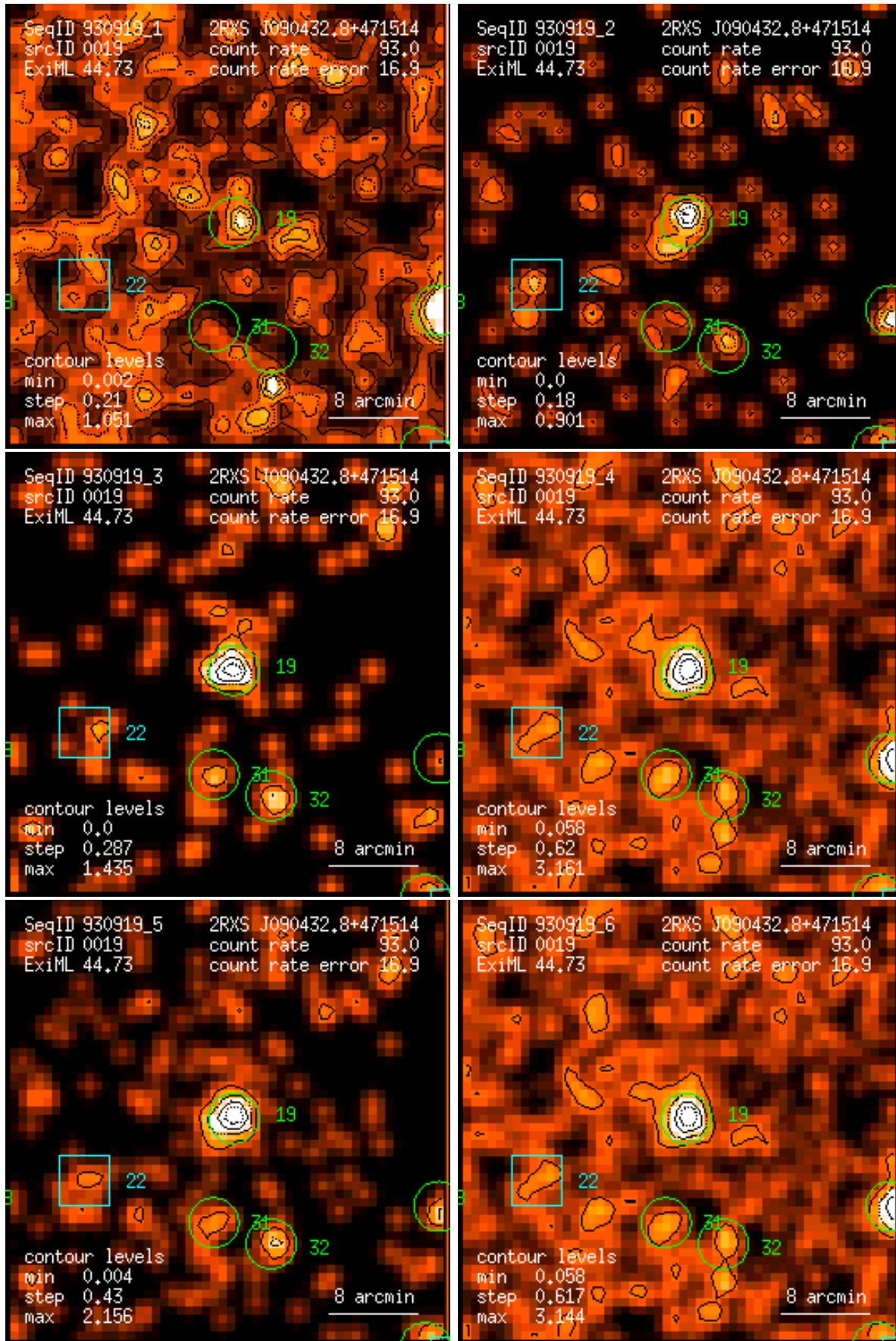
Figure 19: RASS 930919: detection 0019: band rate images, Gaussian filter: (1) PSPC channels 11 – 41, (2) 52 – 90, (3) 91 – 201, (4) 11 – 235, (5) 52 – 201, (6) 11 – 201. Broad band rates in counts/ks. Band rate contour levels in counts/ks/arcmin 2 .
