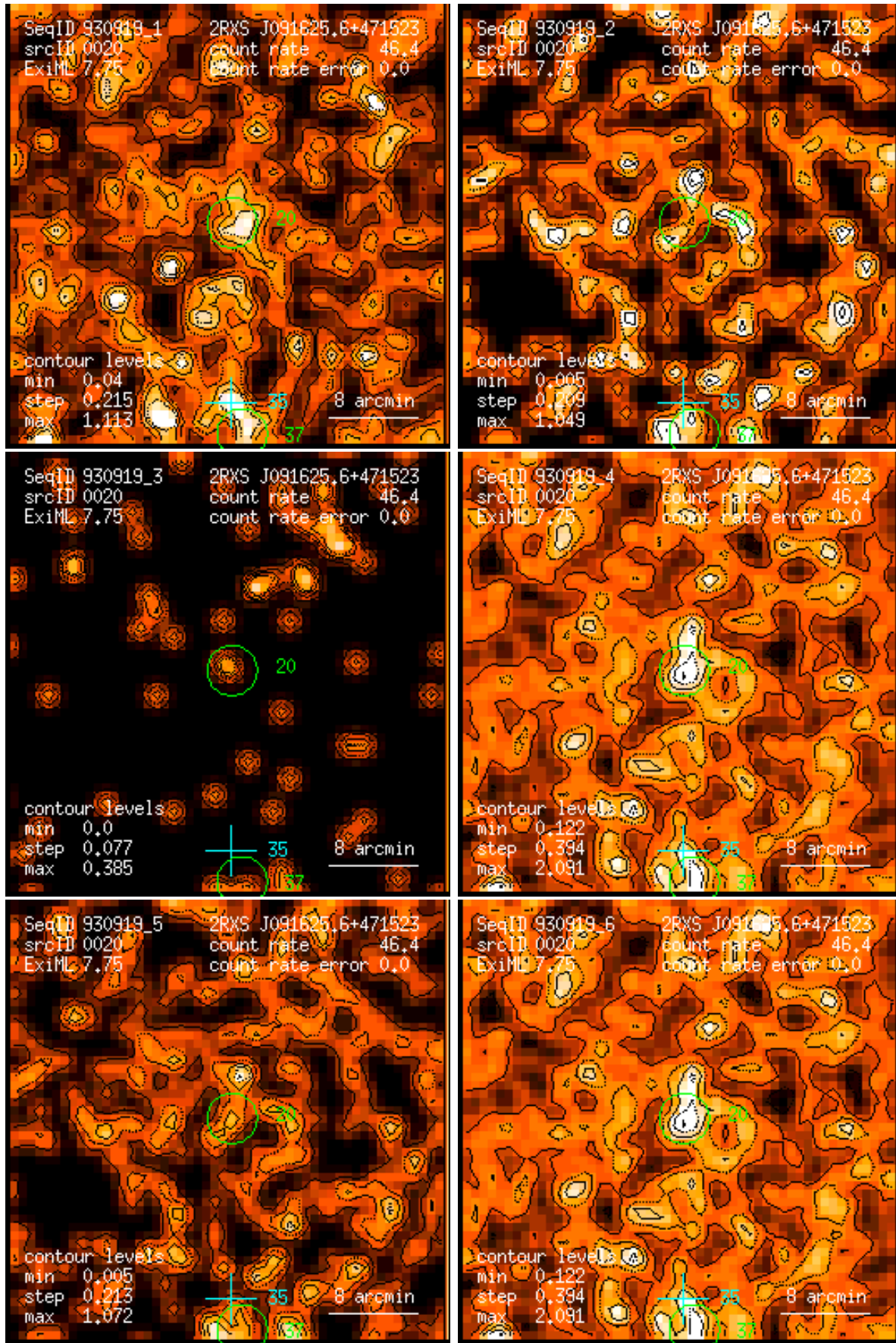
Figure 20: RASS 930919: detection 0020: band rate images, Gaussian filter: (1) PSPC channels 11 – 41, (2) 52 – 90, (3) 91 – 201, (4) 11 – 235, (5) 52 – 201, (6) 11 – 201. Broad band rates in counts/ks. Band rate contour levels in counts/ks/arcmin 2 .
