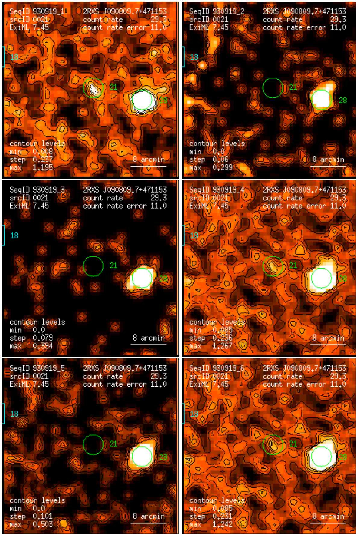
Figure 21: RASS 930919: detection 0021: band rate images, Gaussian filter: (1) PSPC channels 11 – 41, (2) 52 – 90, (3) 91 – 201, (4) 11 – 235, (5) 52 – 201, (6) 11 – 201. Broad band rates in counts/ks. Band rate contour levels in counts/ks/arcmin 2 .
