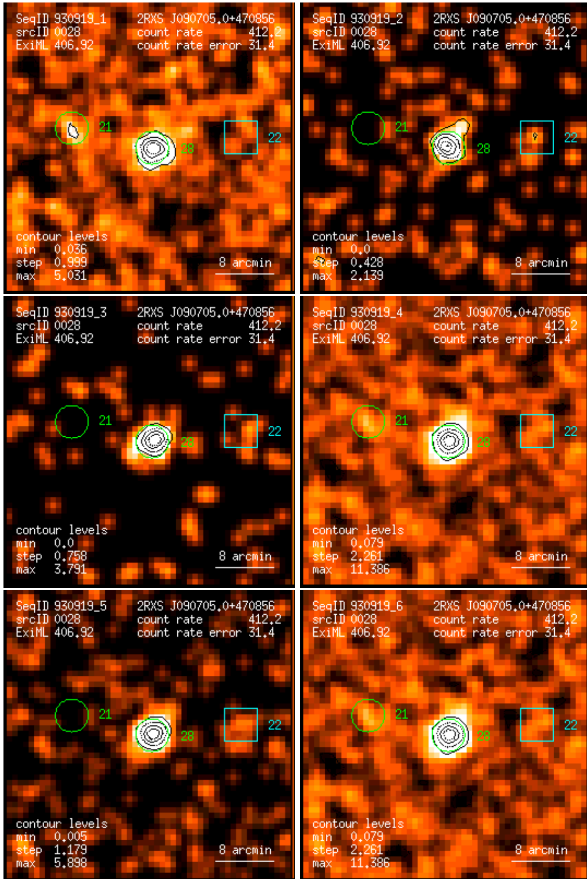
Figure 28: RASS 930919: detection 0028: band rate images, Gaussian filter: (1) PSPC channels 11 – 41, (2) 52 – 90, (3) 91 – 201, (4) 11 – 235, (5) 52 – 201, (6) 11 – 201. Broad band rates in counts/ks. Band rate contour levels in counts/ks/arcmin 2 .
