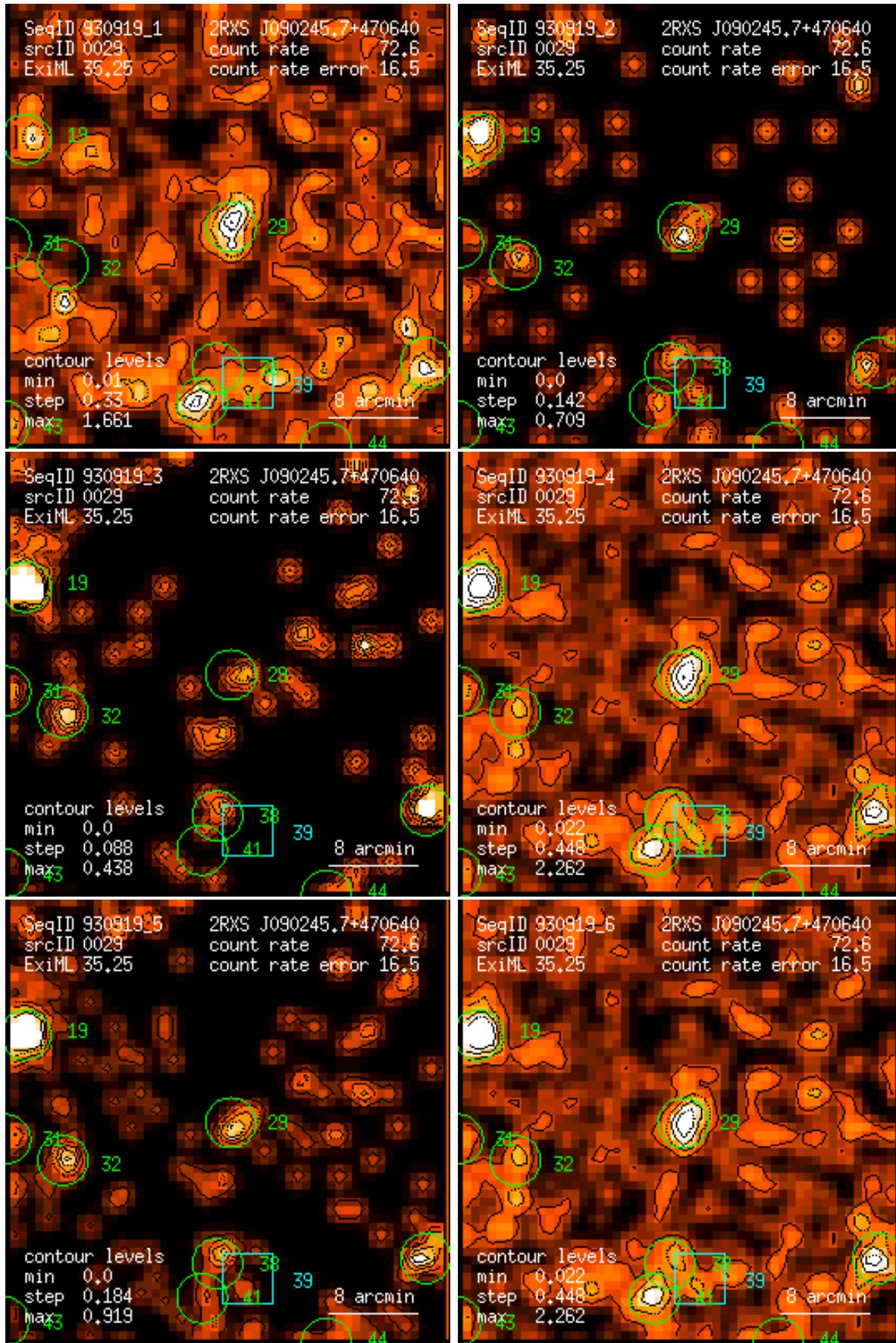
Figure 29: RASS 930919: detection 0029: band rate images, Gaussian filter: (1) PSPC channels 11 – 41, (2) 52 – 90, (3) 91 – 201, (4) 11 – 235, (5) 52 – 201, (6) 11 – 201. Broad band rates in counts/ks. Band rate contour levels in counts/ks/arcmin 2 .
