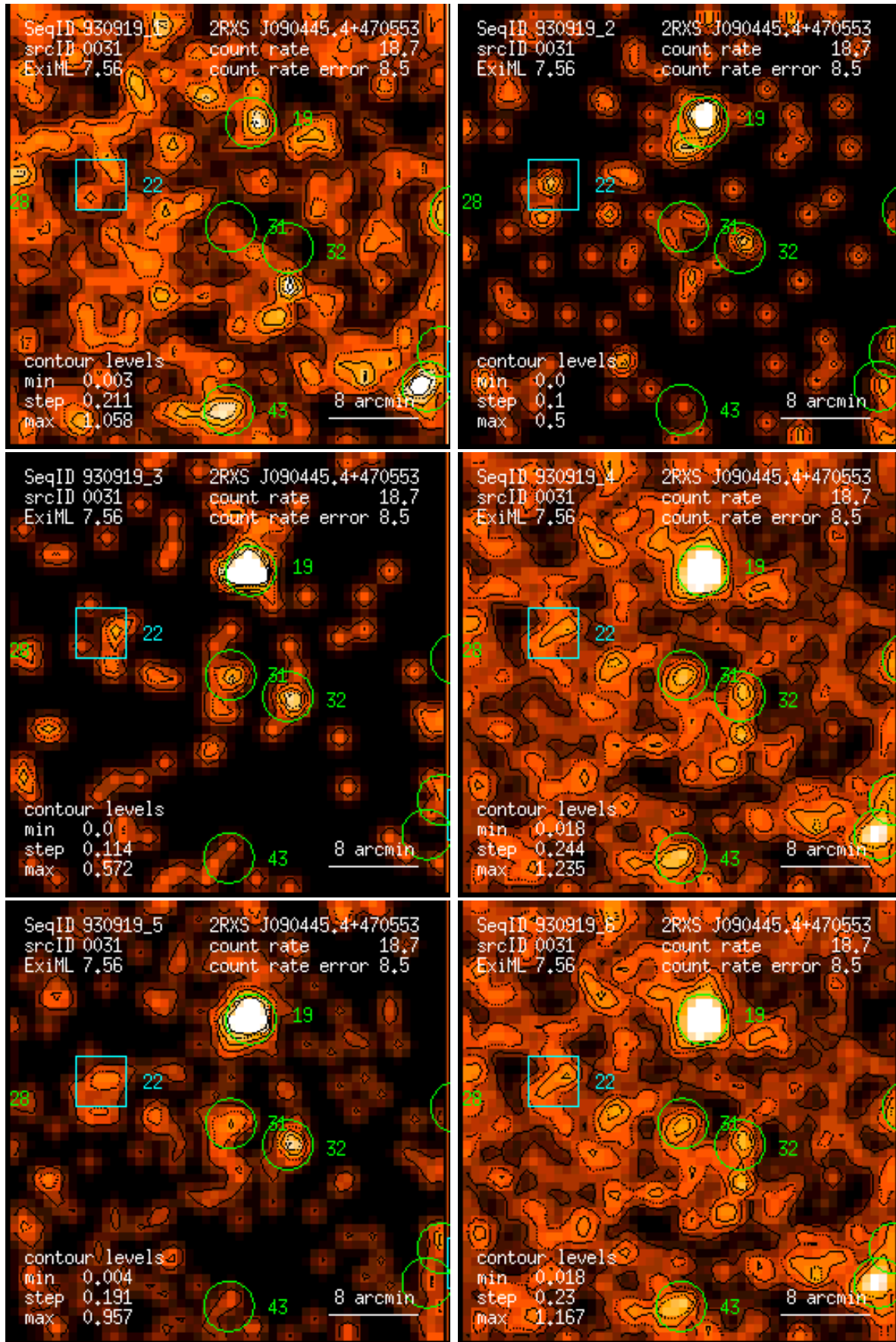
Figure 31: RASS 930919: detection 0031: band rate images, Gaussian filter: (1) PSPC channels 11 – 41, (2) 52 – 90, (3) 91 – 201, (4) 11 – 235, (5) 52 – 201, (6) 11 – 201. Broad band rates in counts/ks. Band rate contour levels in counts/ks/arcmin 2 .
