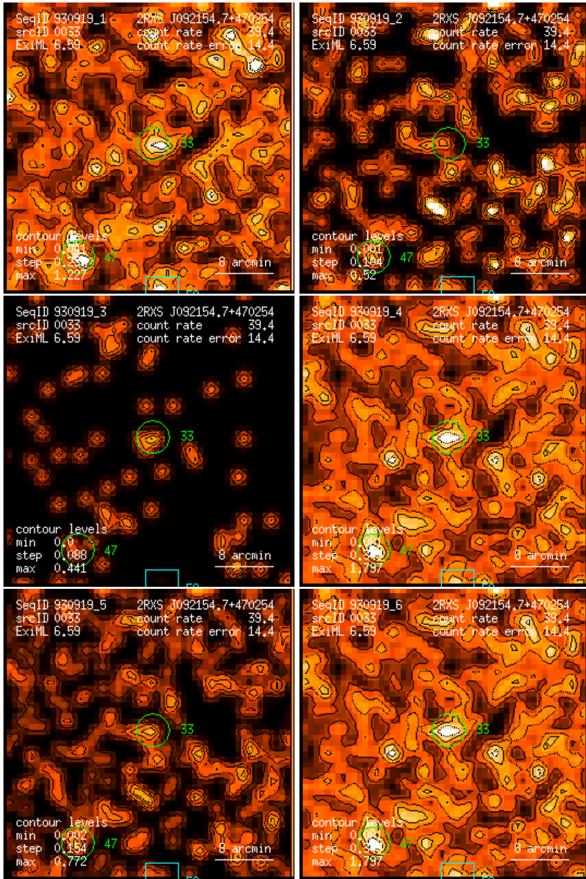
Figure 33: RASS 930919: detection 0033: band rate images, Gaussian filter: (1) PSPC channels 11 – 41, (2) 52 – 90, (3) 91 – 201, (4) 11 – 235, (5) 52 – 201, (6) 11 – 201. Broad band rates in counts/ks. Band rate contour levels in counts/ks/arcmin 2 .
