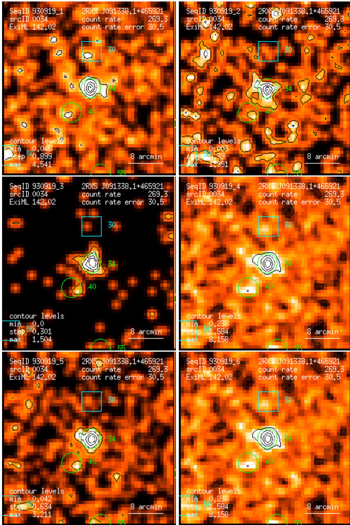
Figure 34: RASS 930919: detection 0034: band rate images, Gaussian filter: (1) PSPC channels 11 – 41, (2) 52 – 90, (3) 91 – 201, (4) 11 – 235, (5) 52 – 201, (6) 11 – 201. Broad band rates in counts/ks. Band rate contour levels in counts/ks/arcmin 2 .
