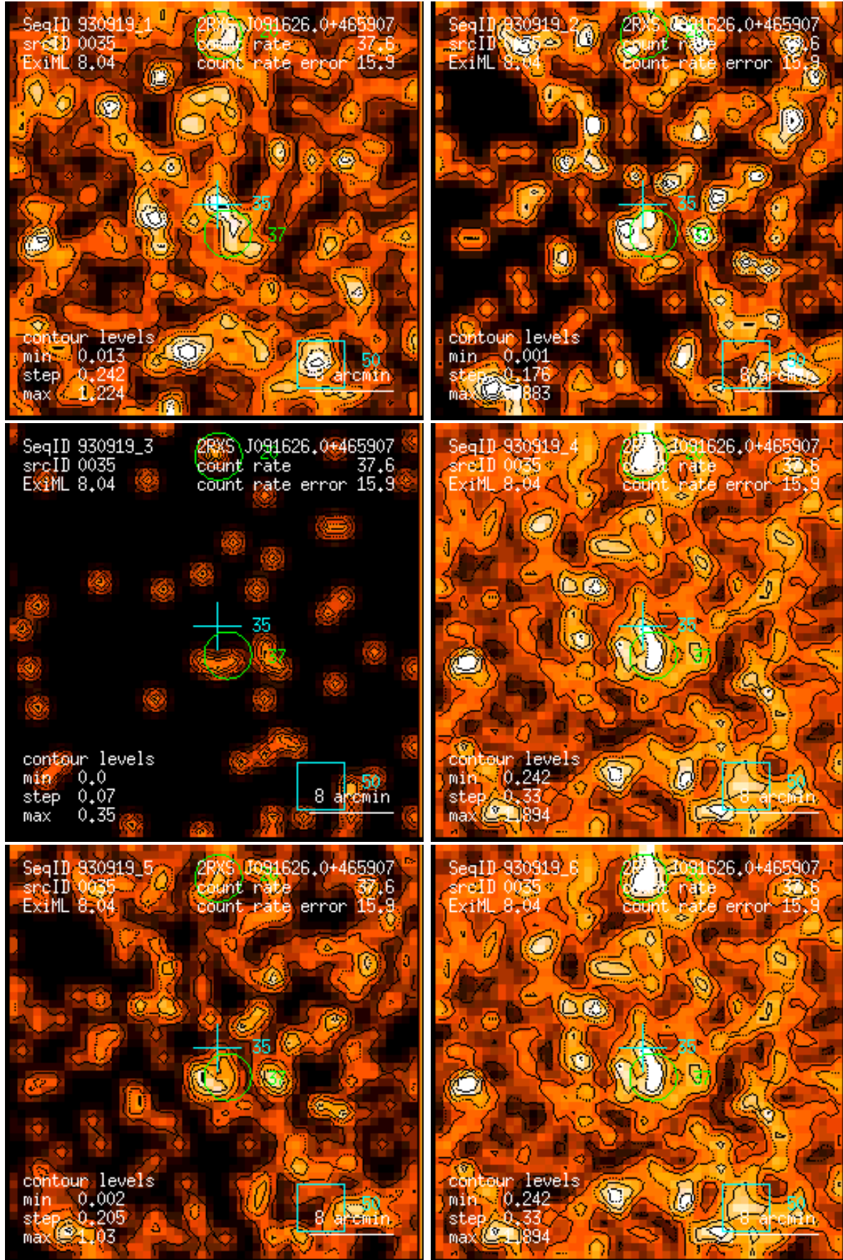
Figure 35: RASS 930919: detection 0035: band rate images, Gaussian filter: (1) PSPC channels 11 – 41, (2) 52 – 90, (3) 91 – 201, (4) 11 – 235, (5) 52 – 201, (6) 11 – 201. Broad band rates in counts/ks. Band rate contour levels in counts/ks/arcmin 2 .
