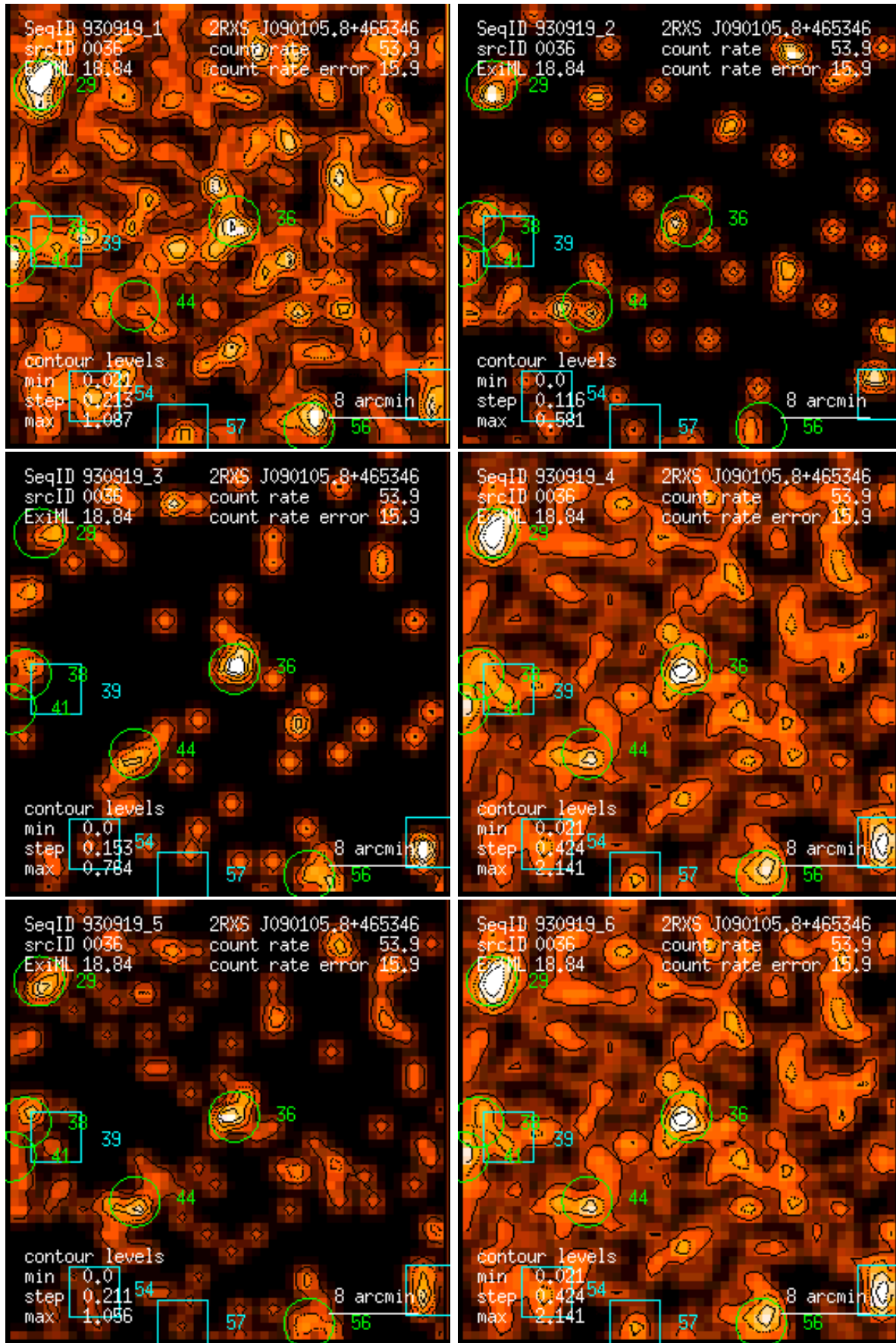
Figure 36: RASS 930919: detection 0036: band rate images, Gaussian filter: (1) PSPC channels 11 – 41, (2) 52 – 90, (3) 91 – 201, (4) 11 – 235, (5) 52 – 201, (6) 11 – 201. Broad band rates in counts/ks. Band rate contour levels in counts/ks/arcmin 2 .
