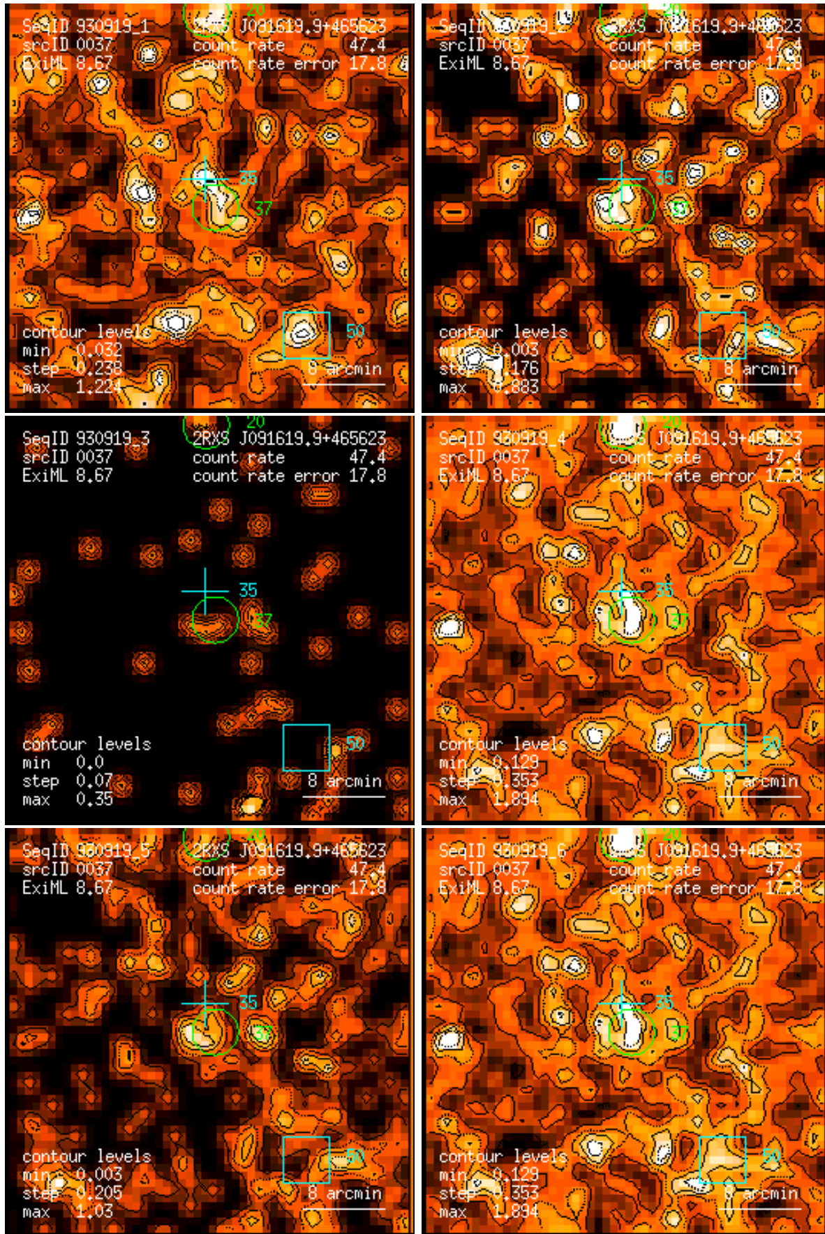
Figure 37: RASS 930919: detection 0037: band rate images, Gaussian filter: (1) PSPC channels 11 – 41, (2) 52 – 90, (3) 91 – 201, (4) 11 – 235, (5) 52 – 201, (6) 11 – 201. Broad band rates in counts/ks. Band rate contour levels in counts/ks/arcmin 2 .
