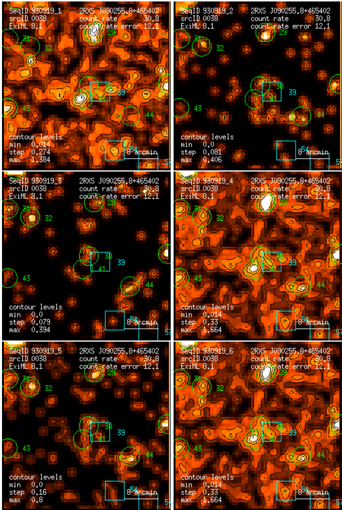
Figure 38: RASS 930919: detection 0038: band rate images, Gaussian filter: (1) PSPC channels 11 – 41, (2) 52 – 90, (3) 91 – 201, (4) 11 – 235, (5) 52 – 201, (6) 11 – 201. Broad band rates in counts/ks. Band rate contour levels in counts/ks/arcmin 2 .
