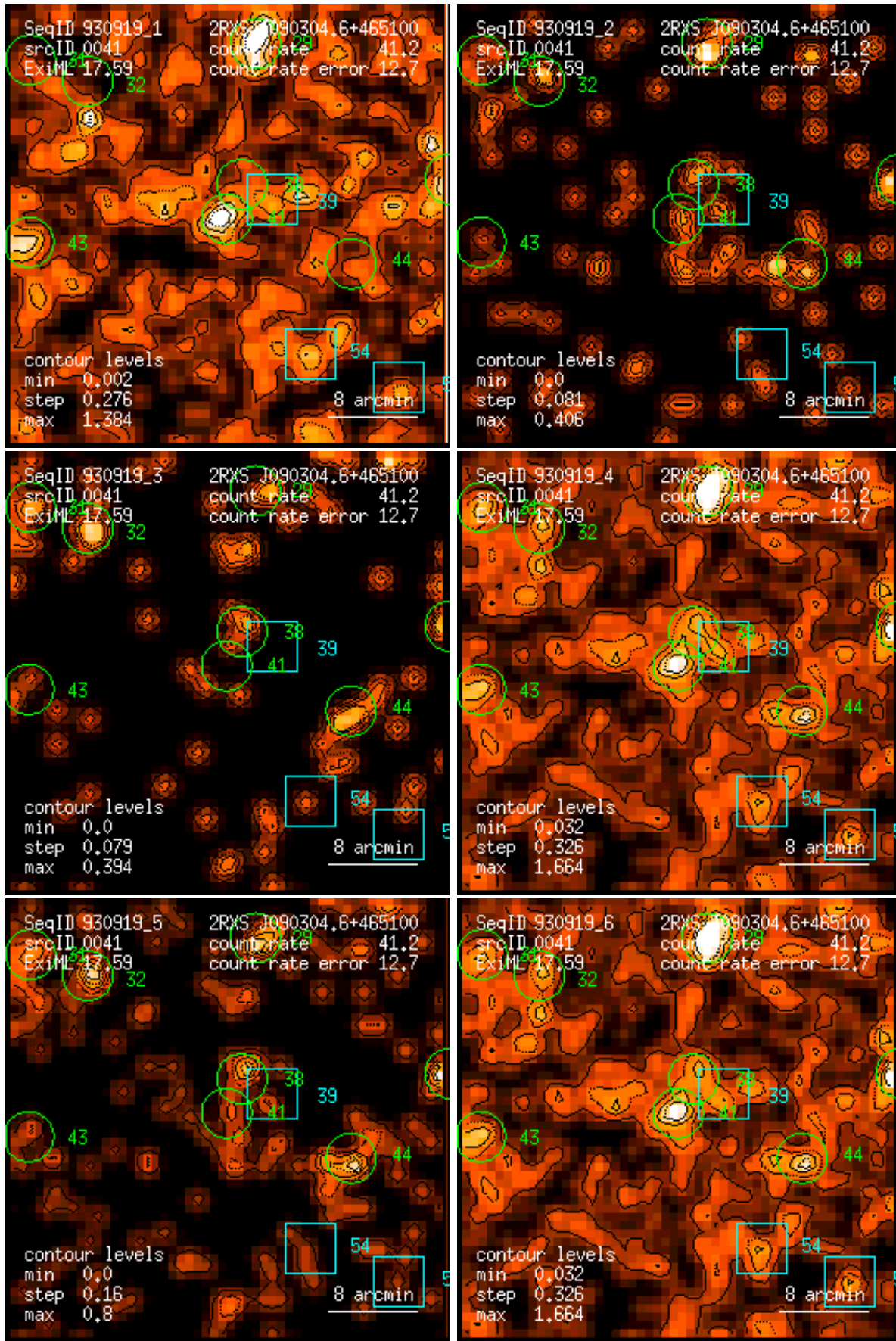
Figure 41: RASS 930919: detection 0041: band rate images, Gaussian filter: (1) PSPC channels 11 – 41, (2) 52 – 90, (3) 91 – 201, (4) 11 – 235, (5) 52 – 201, (6) 11 – 201. Broad band rates in counts/ks. Band rate contour levels in counts/ks/arcmin 2 .
