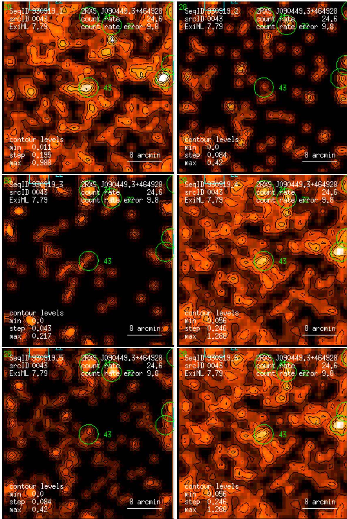
Figure 43: RASS 930919: detection 0043: band rate images, Gaussian filter: (1) PSPC channels 11 – 41, (2) 52 – 90, (3) 91 – 201, (4) 11 – 235, (5) 52 – 201, (6) 11 – 201. Broad band rates in counts/ks. Band rate contour levels in counts/ks/arcmin 2 .
