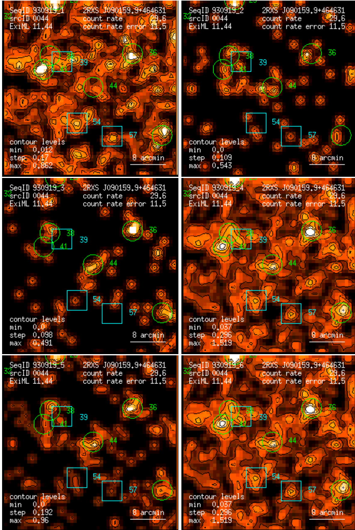
Figure 44: RASS 930919: detection 0044: band rate images, Gaussian filter: (1) PSPC channels 11 – 41, (2) 52 – 90, (3) 91 – 201, (4) 11 – 235, (5) 52 – 201, (6) 11 – 201. Broad band rates in counts/ks. Band rate contour levels in counts/ks/arcmin 2 .
