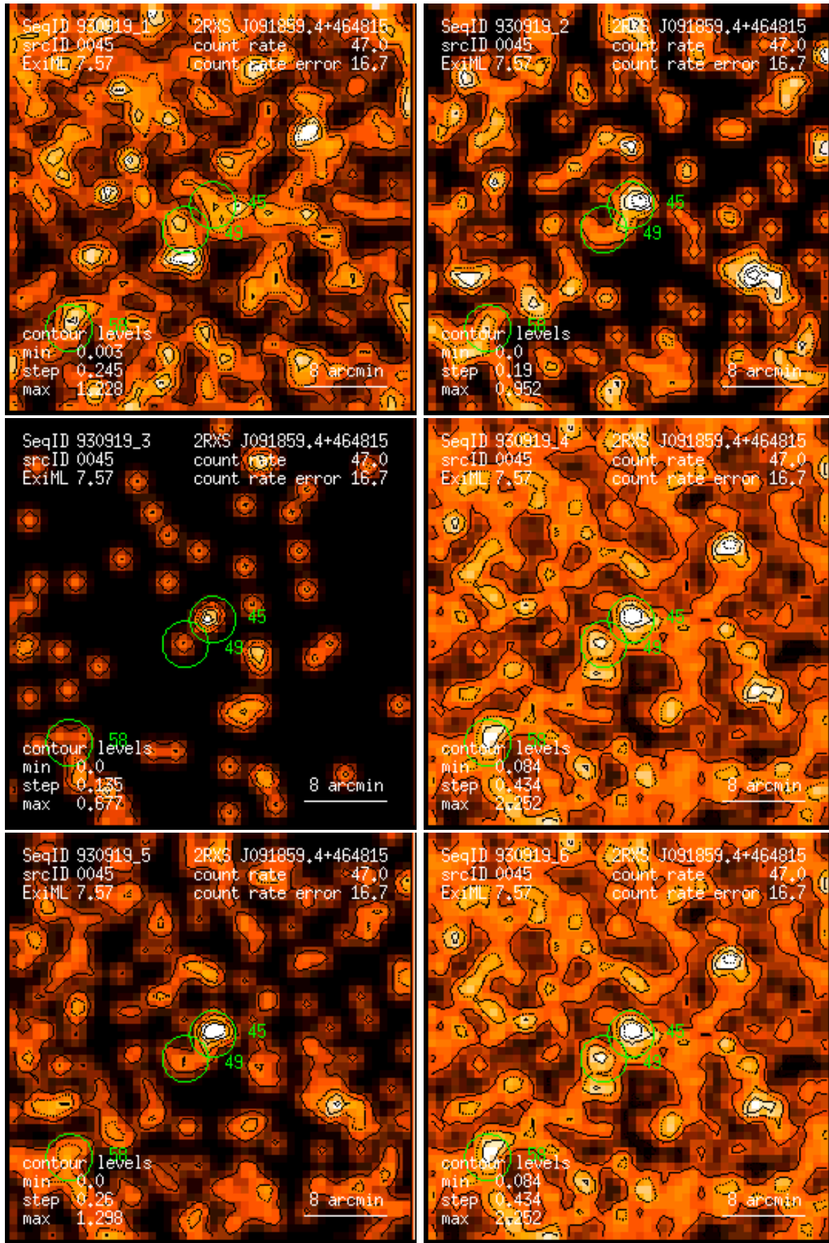
Figure 45: RASS 930919: detection 0045: band rate images, Gaussian filter: (1) PSPC channels 11 – 41, (2) 52 – 90, (3) 91 – 201, (4) 11 – 235, (5) 52 – 201, (6) 11 – 201. Broad band rates in counts/ks. Band rate contour levels in counts/ks/arcmin 2 .
