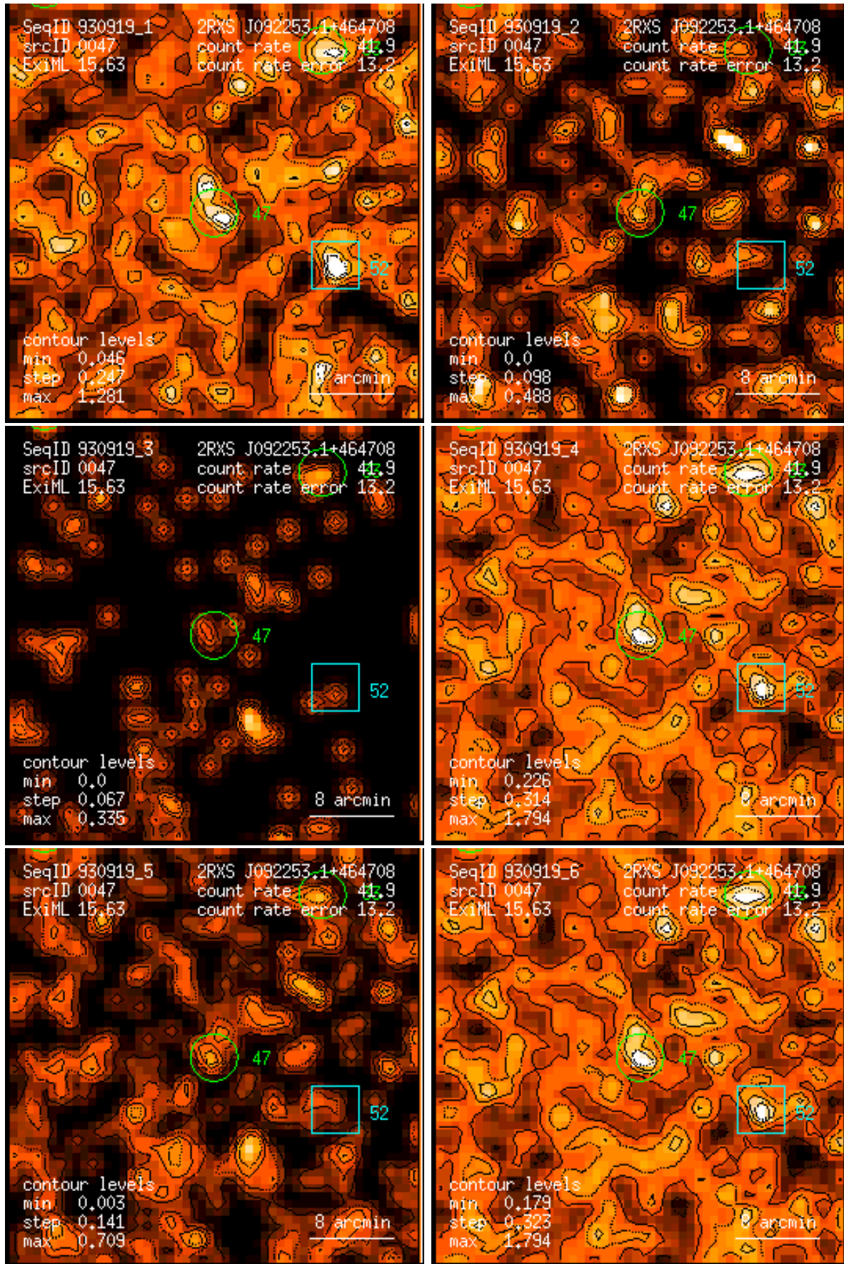
Figure 47: RASS 930919: detection 0047: band rate images, Gaussian filter: (1) PSPC channels 11 – 41, (2) 52 – 90, (3) 91 – 201, (4) 11 – 235, (5) 52 – 201, (6) 11 – 201. Broad band rates in counts/ks. Band rate contour levels in counts/ks/arcmin 2 .
