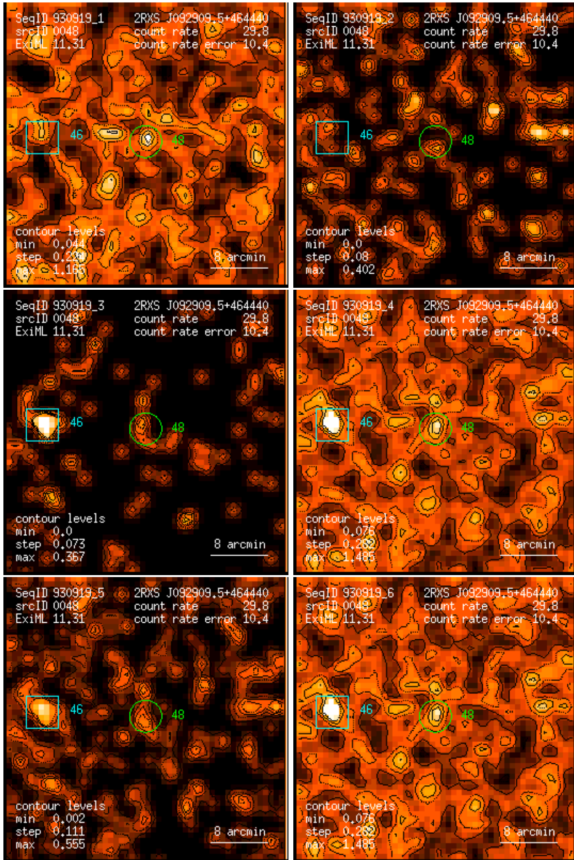
Figure 48: RASS 930919: detection 0048: band rate images, Gaussian filter: (1) PSPC channels 11 – 41, (2) 52 – 90, (3) 91 – 201, (4) 11 – 235, (5) 52 – 201, (6) 11 – 201. Broad band rates in counts/ks. Band rate contour levels in counts/ks/arcmin 2 .
