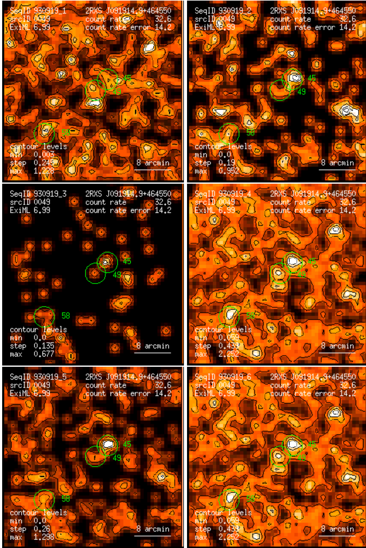
Figure 49: RASS 930919: detection 0049: band rate images, Gaussian filter: (1) PSPC channels 11 – 41, (2) 52 – 90, (3) 91 – 201, (4) 11 – 235, (5) 52 – 201, (6) 11 – 201. Broad band rates in counts/ks. Band rate contour levels in counts/ks/arcmin 2 .
