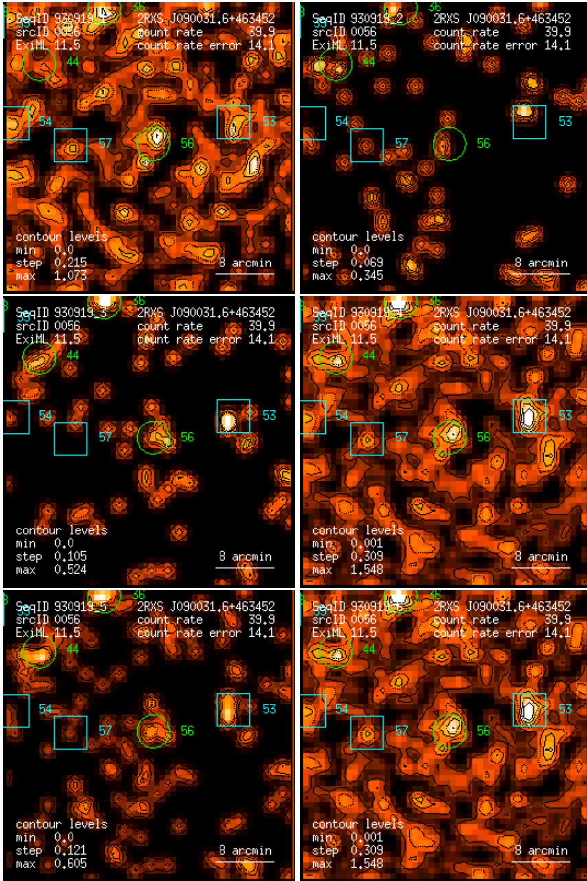
Figure 56: RASS 930919: detection 0056: band rate images, Gaussian filter: (1) PSPC channels 11 – 41, (2) 52 – 90, (3) 91 – 201, (4) 11 – 235, (5) 52 – 201, (6) 11 – 201. Broad band rates in counts/ks. Band rate contour levels in counts/ks/arcmin 2 .
