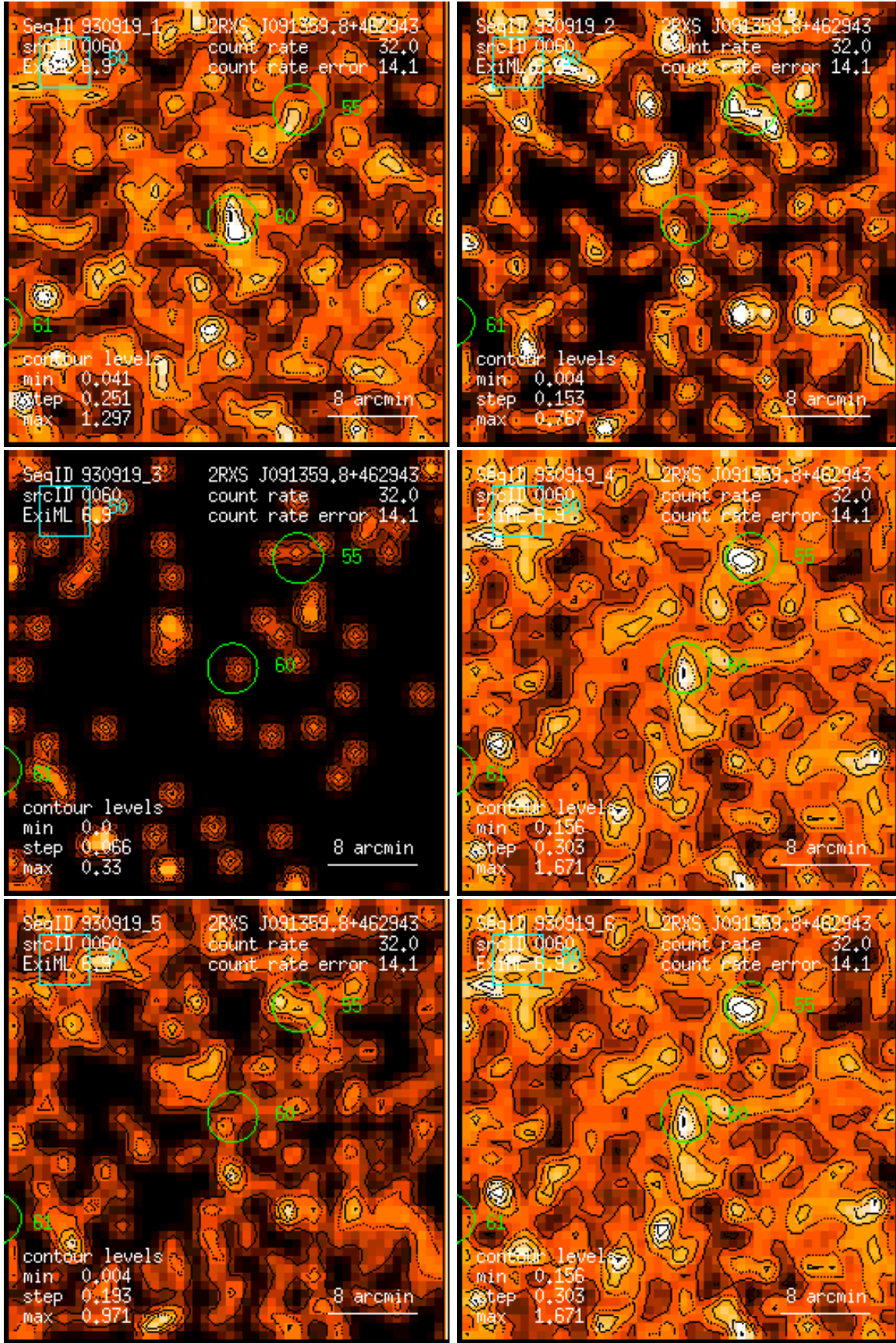
Figure 60: RASS 930919: detection 0060: band rate images, Gaussian filter: (1) PSPC channels 11 – 41, (2) 52 – 90, (3) 91 – 201, (4) 11 – 235, (5) 52 – 201, (6) 11 – 201. Broad band rates in counts/ks. Band rate contour levels in counts/ks/arcmin 2 .
