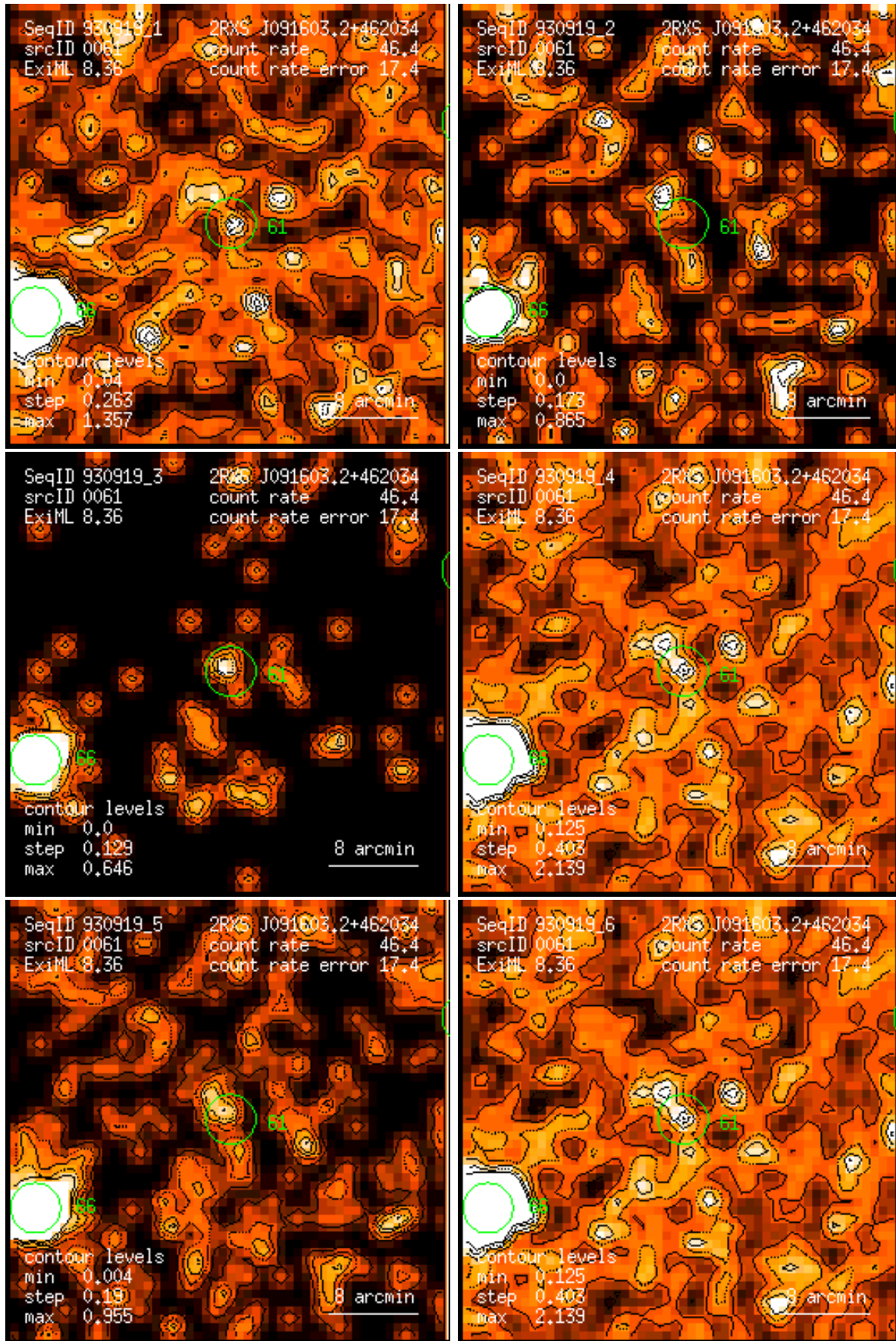
Figure 61: RASS 930919: detection 0061: band rate images, Gaussian filter: (1) PSPC channels 11 – 41, (2) 52 – 90, (3) 91 – 201, (4) 11 – 235, (5) 52 – 201, (6) 11 – 201. Broad band rates in counts/ks. Band rate contour levels in counts/ks/arcmin 2 .
