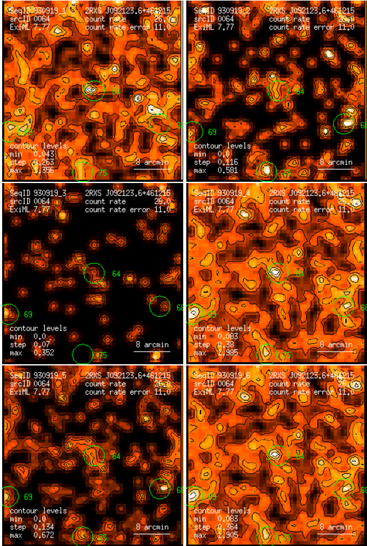
Figure 64: RASS 930919: detection 0064: band rate images, Gaussian filter: (1) PSPC channels 11 – 41, (2) 52 – 90, (3) 91 – 201, (4) 11 – 235, (5) 52 – 201, (6) 11 – 201. Broad band rates in counts/ks. Band rate contour levels in counts/ks/arcmin 2 .
