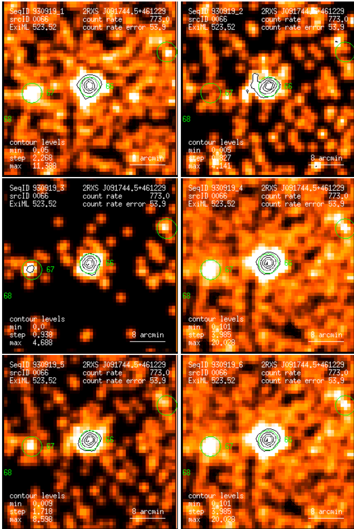
Figure 66: RASS 930919: detection 0066: band rate images, Gaussian filter: (1) PSPC channels 11 – 41, (2) 52 – 90, (3) 91 – 201, (4) 11 – 235, (5) 52 – 201, (6) 11 – 201. Broad band rates in counts/ks. Band rate contour levels in counts/ks/arcmin 2 .
