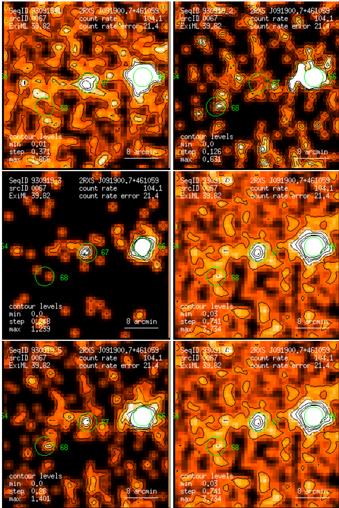
Figure 67: RASS 930919: detection 0067: band rate images, Gaussian filter: (1) PSPC channels 11 – 41, (2) 52 – 90, (3) 91 – 201, (4) 11 – 235, (5) 52 – 201, (6) 11 – 201. Broad band rates in counts/ks. Band rate contour levels in counts/ks/arcmin 2 .
