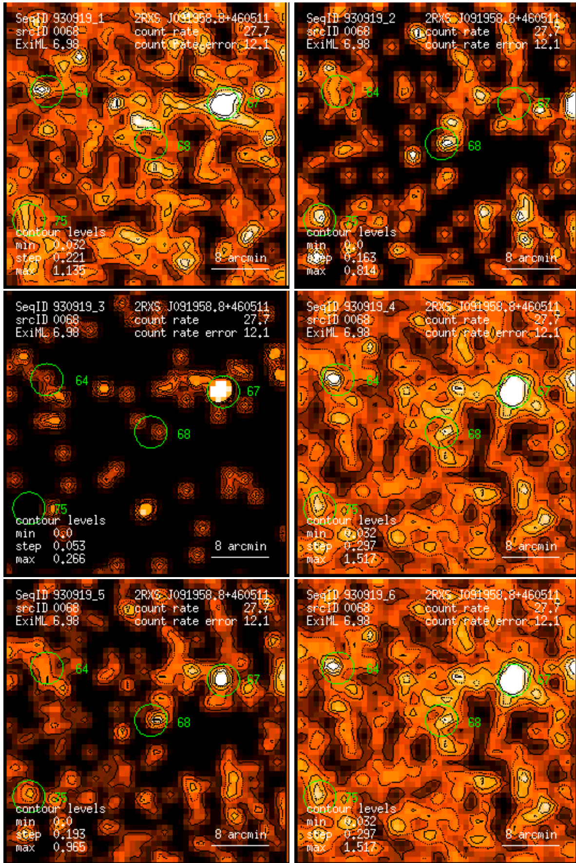
Figure 68: RASS 930919: detection 0068: band rate images, Gaussian filter: (1) PSPC channels 11 – 41, (2) 52 – 90, (3) 91 – 201, (4) 11 – 235, (5) 52 – 201, (6) 11 – 201. Broad band rates in counts/ks. Band rate contour levels in counts/ks/arcmin 2 .
