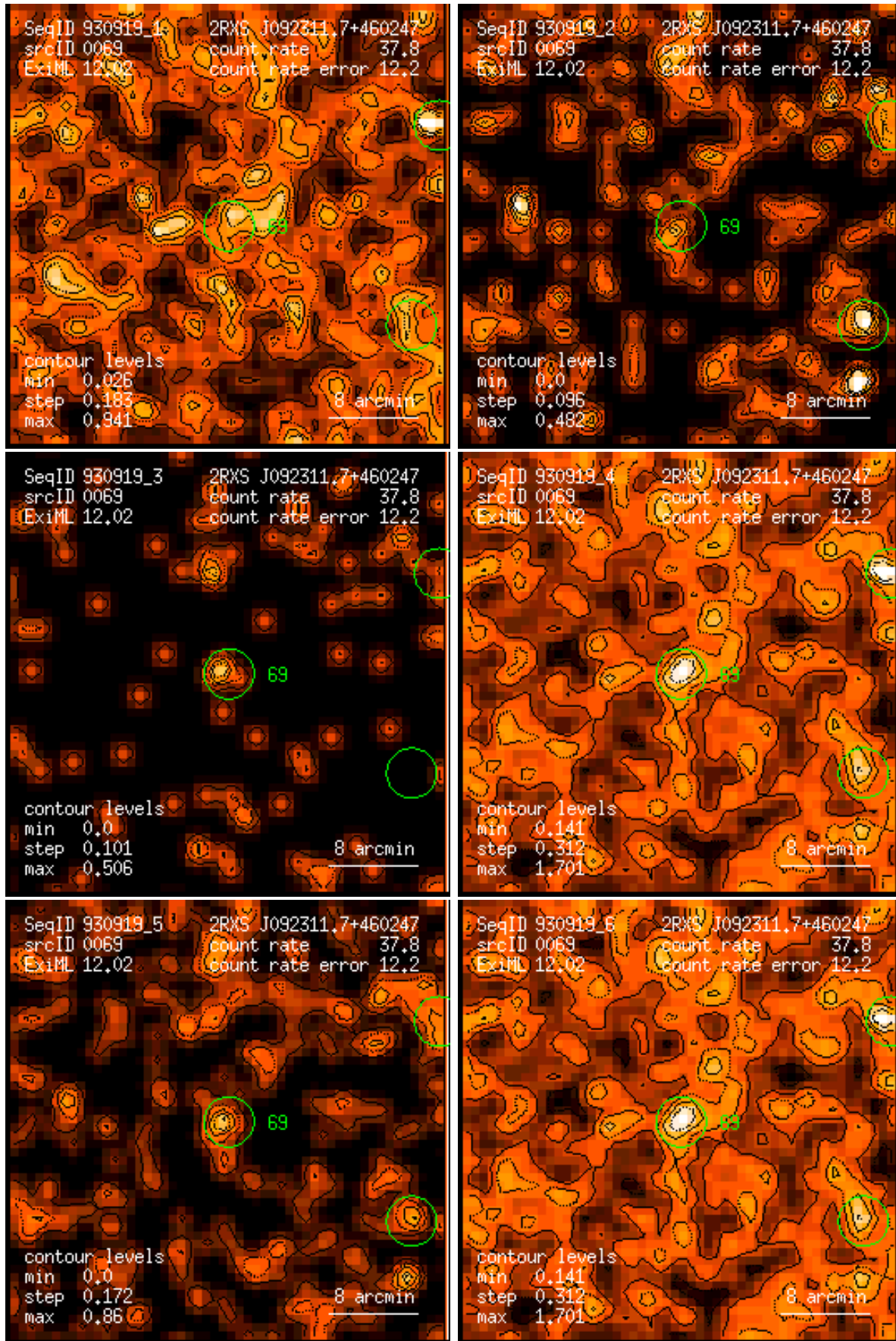
Figure 69: RASS 930919: detection 0069: band rate images, Gaussian filter: (1) PSPC channels 11 – 41, (2) 52 – 90, (3) 91 – 201, (4) 11 – 235, (5) 52 – 201, (6) 11 – 201. Broad band rates in counts/ks. Band rate contour levels in counts/ks/arcmin 2 .
