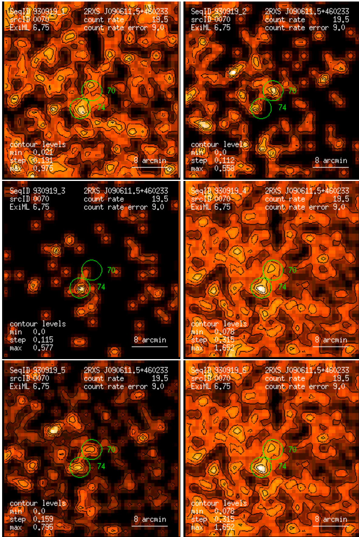
Figure 70: RASS 930919: detection 0070: band rate images, Gaussian filter: (1) PSPC channels 11 – 41, (2) 52 – 90, (3) 91 – 201, (4) 11 – 235, (5) 52 – 201, (6) 11 – 201. Broad band rates in counts/ks. Band rate contour levels in counts/ks/arcmin 2 .
