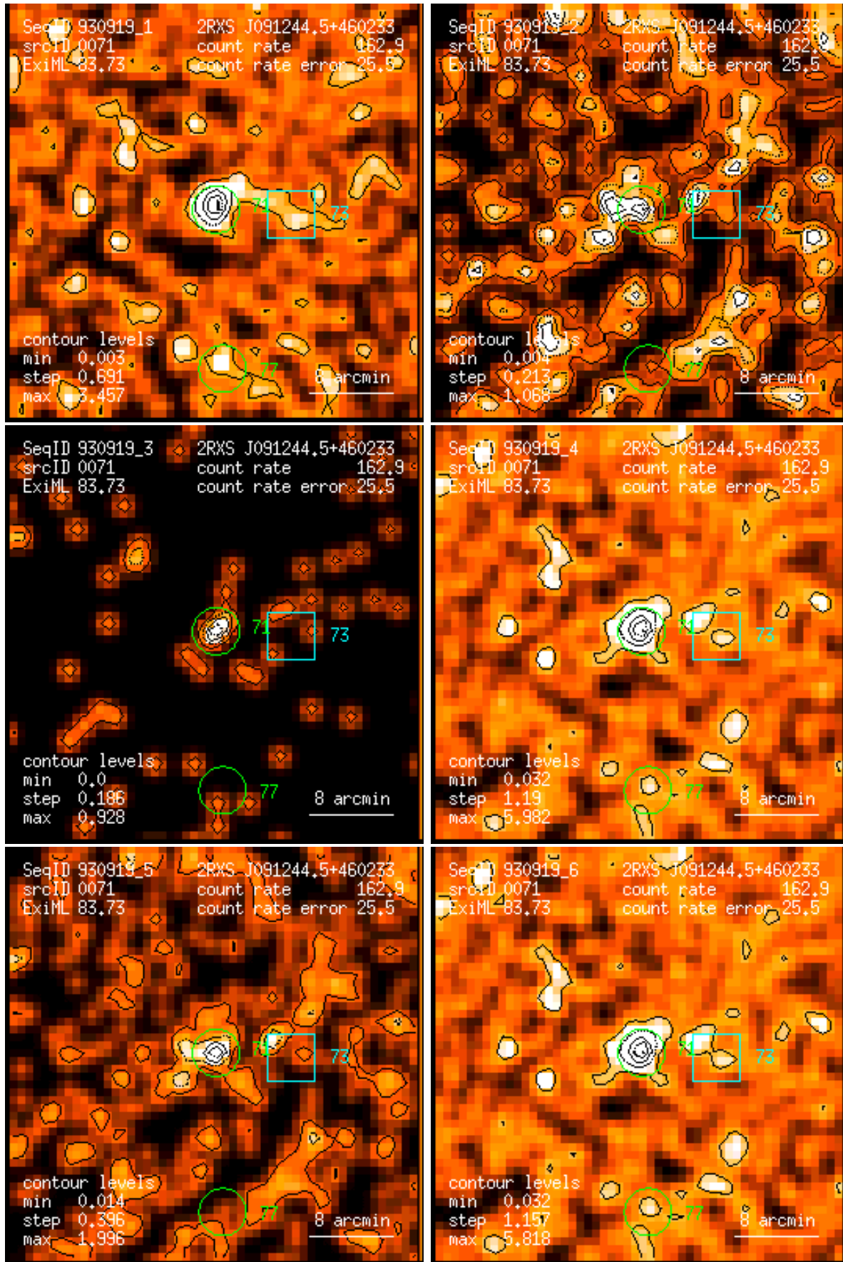
Figure 71: RASS 930919: detection 0071: band rate images, Gaussian filter: (1) PSPC channels 11 – 41, (2) 52 – 90, (3) 91 – 201, (4) 11 – 235, (5) 52 – 201, (6) 11 – 201. Broad band rates in counts/ks. Band rate contour levels in counts/ks/arcmin 2 .
