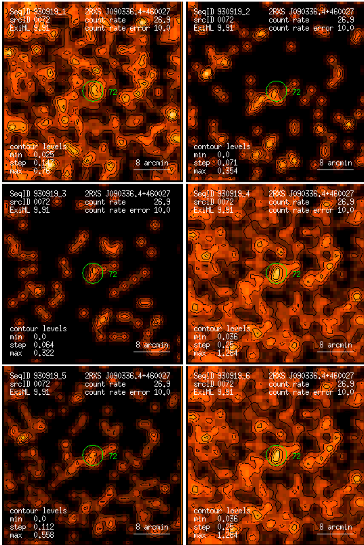
Figure 72: RASS 930919: detection 0072: band rate images, Gaussian filter: (1) PSPC channels 11 – 41, (2) 52 – 90, (3) 91 – 201, (4) 11 – 235, (5) 52 – 201, (6) 11 – 201. Broad band rates in counts/ks. Band rate contour levels in counts/ks/arcmin 2 .
