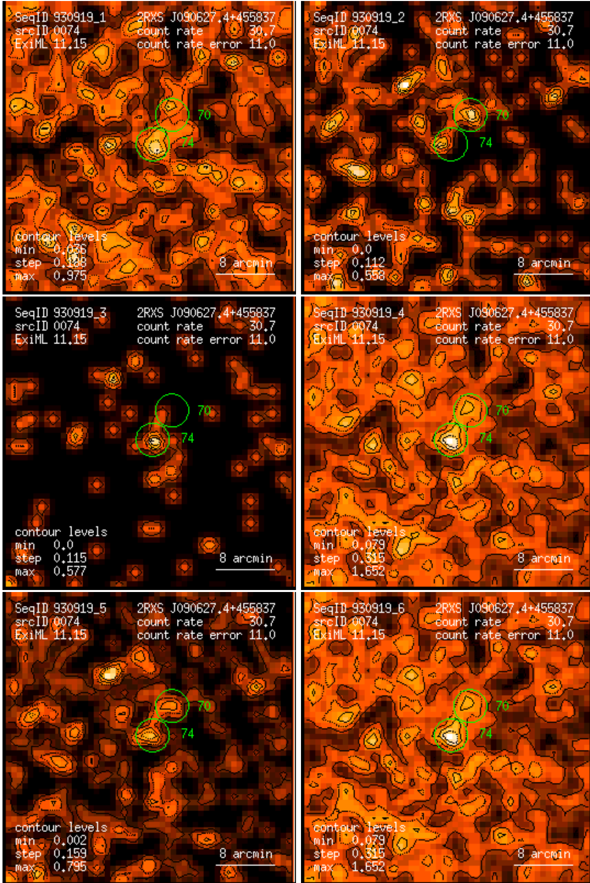
Figure 74: RASS 930919: detection 0074: band rate images, Gaussian filter: (1) PSPC channels 11 – 41, (2) 52 – 90, (3) 91 – 201, (4) 11 – 235, (5) 52 – 201, (6) 11 – 201. Broad band rates in counts/ks. Band rate contour levels in counts/ks/arcmin 2 .
