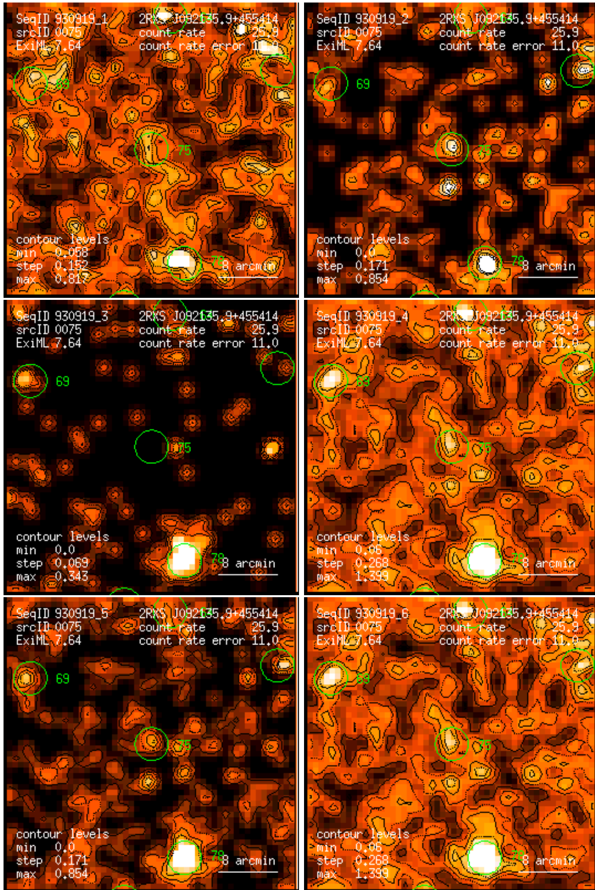
Figure 75: RASS 930919: detection 0075: band rate images, Gaussian filter: (1) PSPC channels 11 – 41, (2) 52 – 90, (3) 91 – 201, (4) 11 – 235, (5) 52 – 201, (6) 11 – 201. Broad band rates in counts/ks. Band rate contour levels in counts/ks/arcmin 2 .
