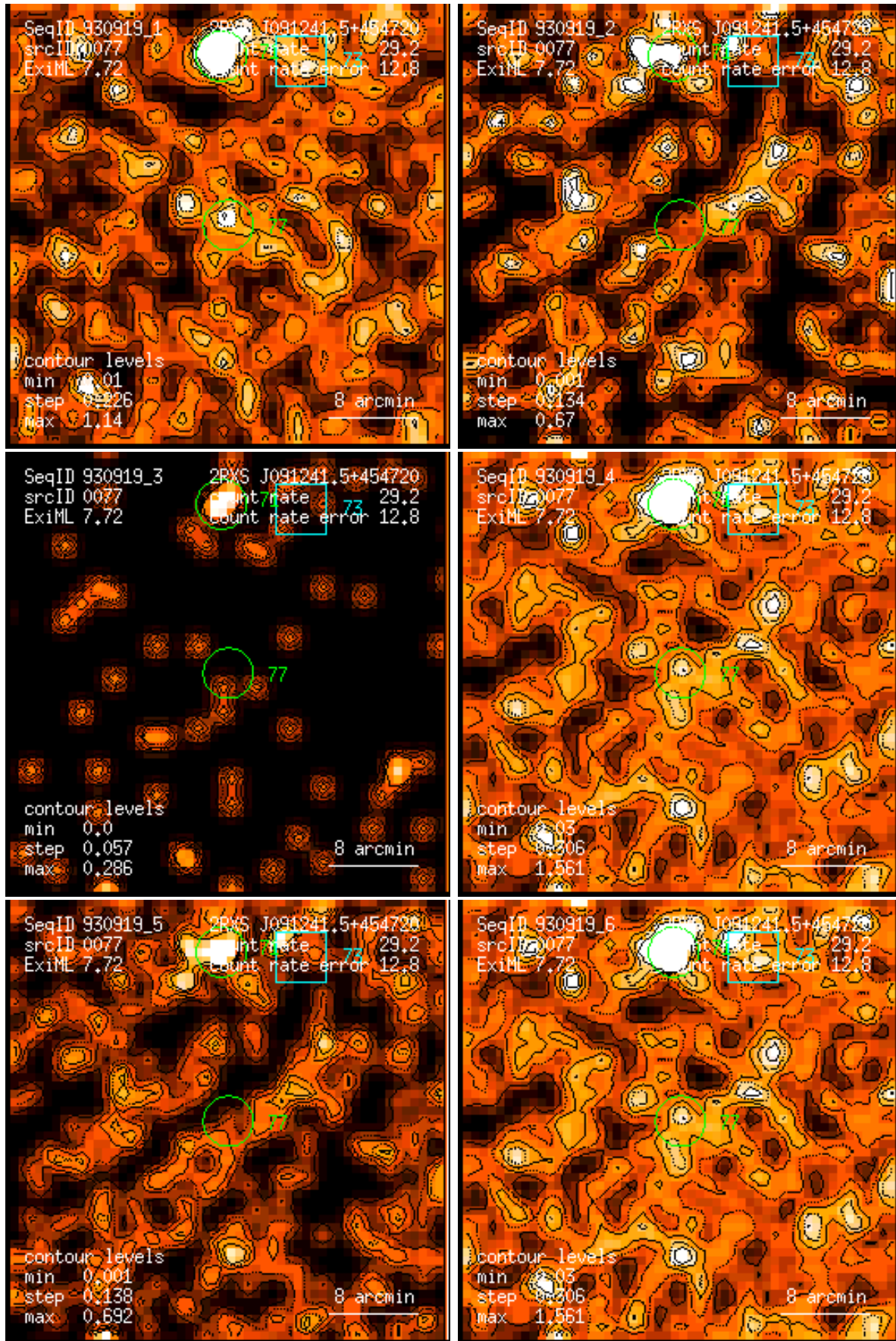
Figure 77: RASS 930919: detection 0077: band rate images, Gaussian filter: (1) PSPC channels 11 – 41, (2) 52 – 90, (3) 91 – 201, (4) 11 – 235, (5) 52 – 201, (6) 11 – 201. Broad band rates in counts/ks. Band rate contour levels in counts/ks/arcmin 2 .
